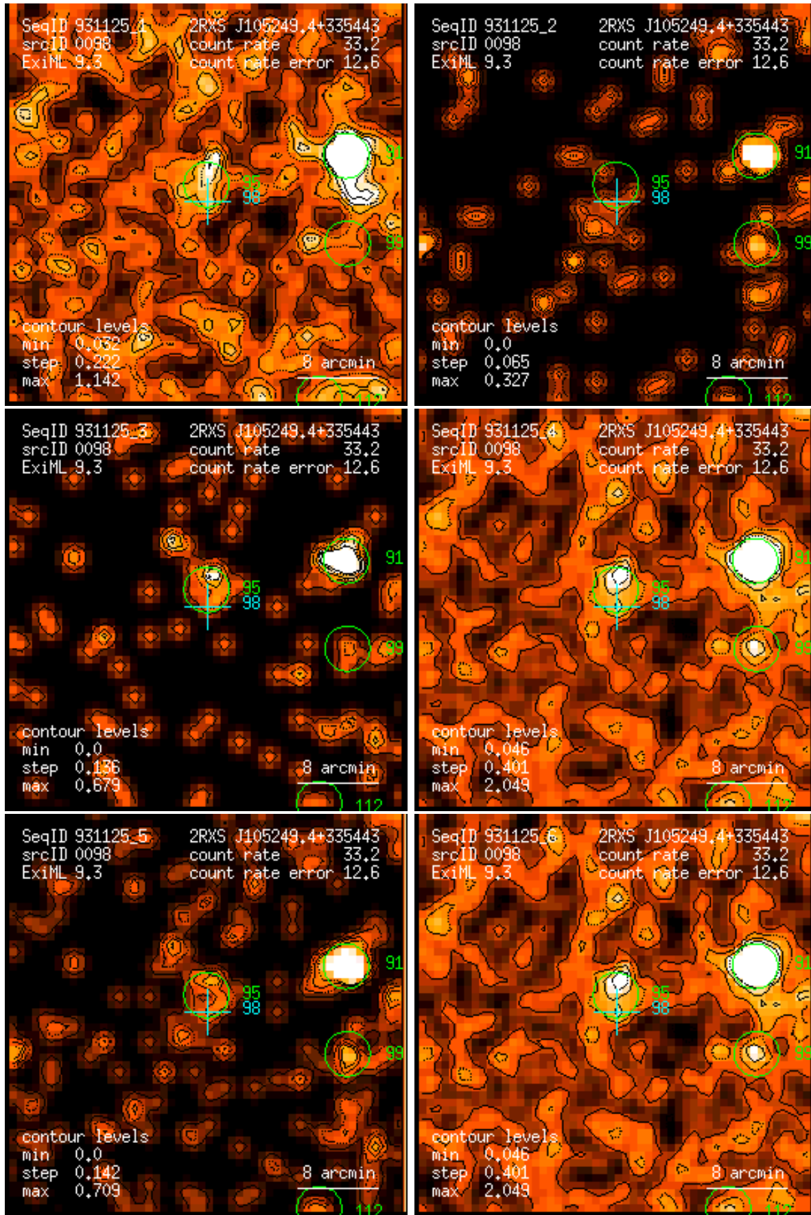
Figure 98: RASS 931125: detection 0098: band rate images, Gaussian filter: (1) PSPC channels 11 – 41, (2) 52 – 90, (3) 91 – 201, (4) 11 – 235, (5) 52 – 201, (6) 11 – 201. Broad band rates in counts/ks. Band rate contour levels in counts/ks/arcmin 2 .
