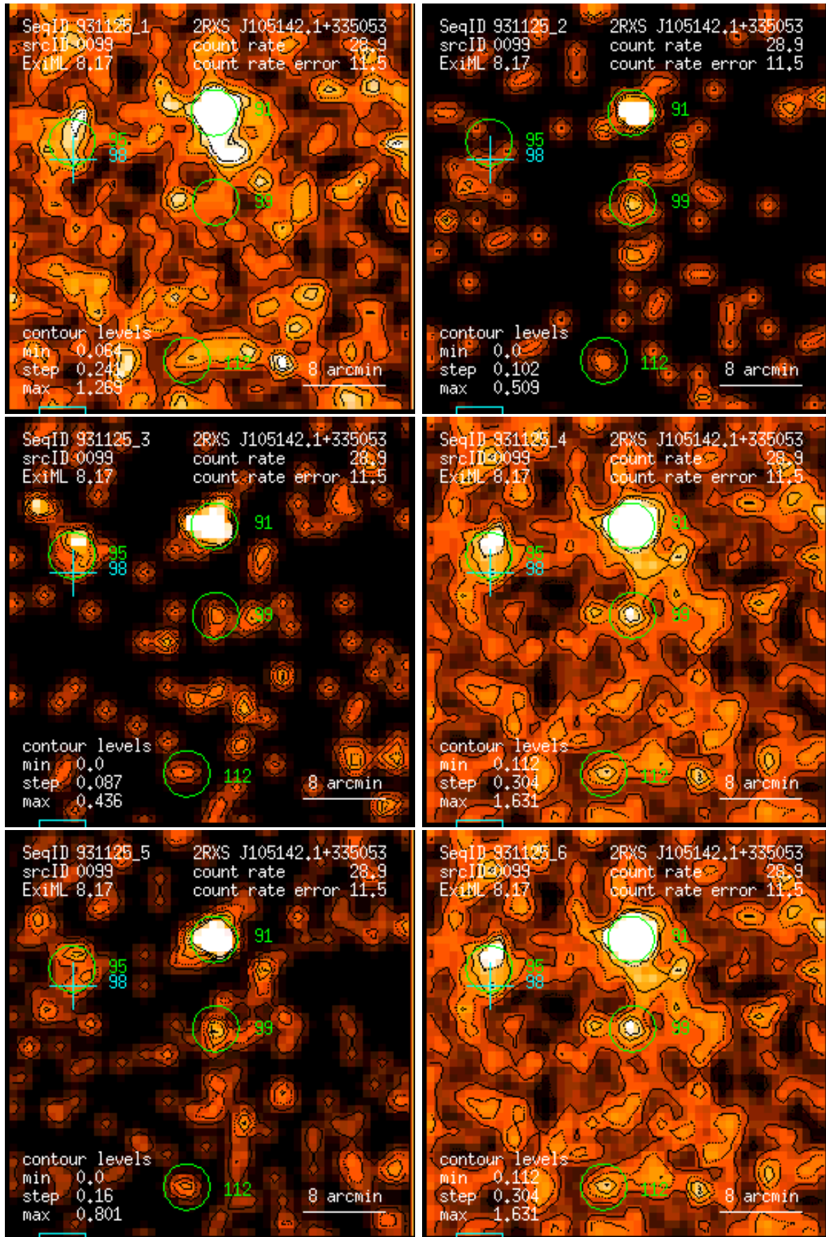
Figure 99: RASS 931125: detection 0099: band rate images, Gaussian filter: (1) PSPC channels 11 – 41, (2) 52 – 90, (3) 91 – 201, (4) 11 – 235, (5) 52 – 201, (6) 11 – 201. Broad band rates in counts/ks. Band rate contour levels in counts/ks/arcmin 2 .
