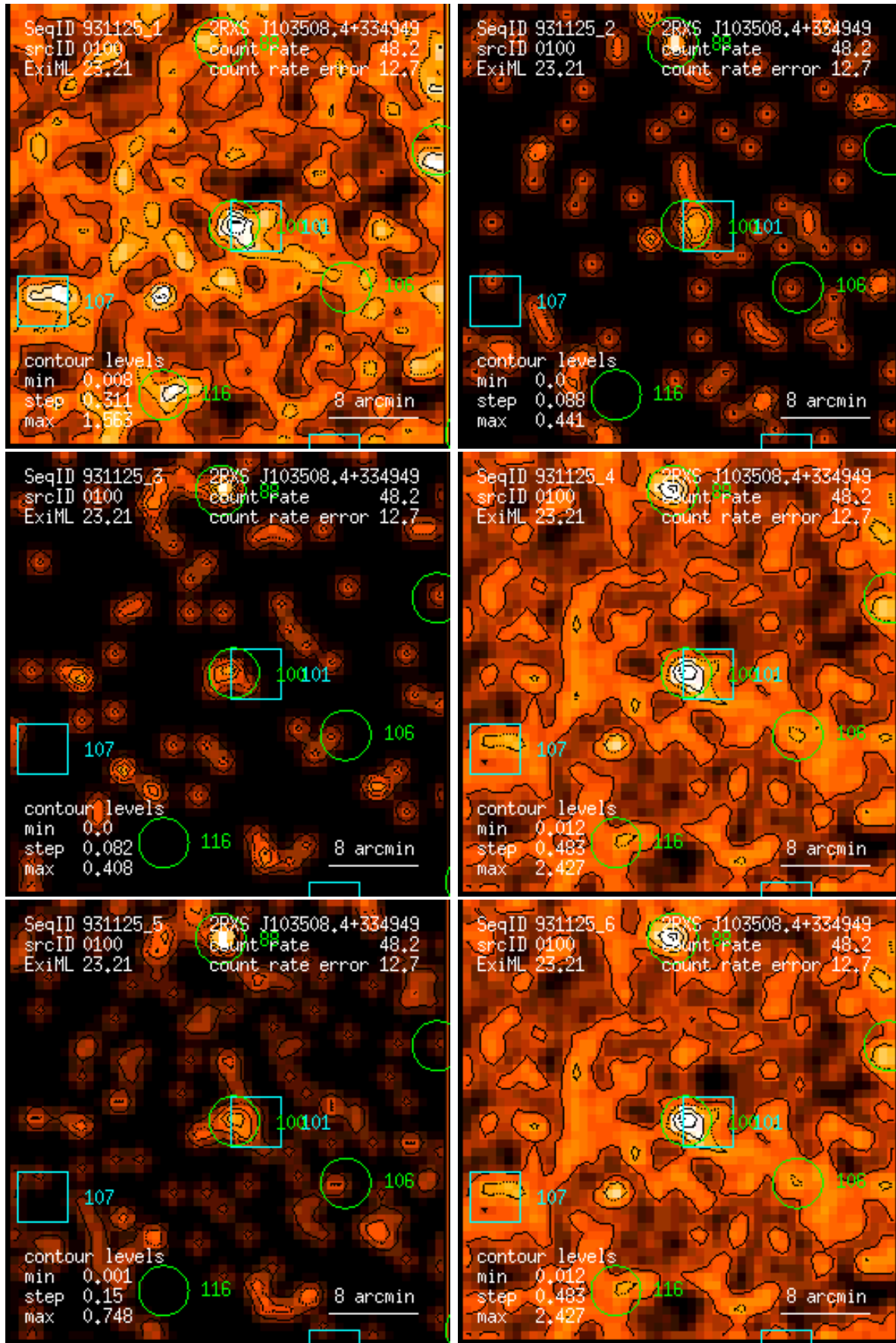
Figure 100: RASS 931125: detection 0100: band rate images, Gaussian filter: (1) PSPC channels 11 – 41, (2) 52 – 90, (3) 91 – 201, (4) 11 – 235, (5) 52 – 201, (6) 11 – 201. Broad band rates in counts/ks. Band rate contour levels in counts/ks/arcmin 2 .
