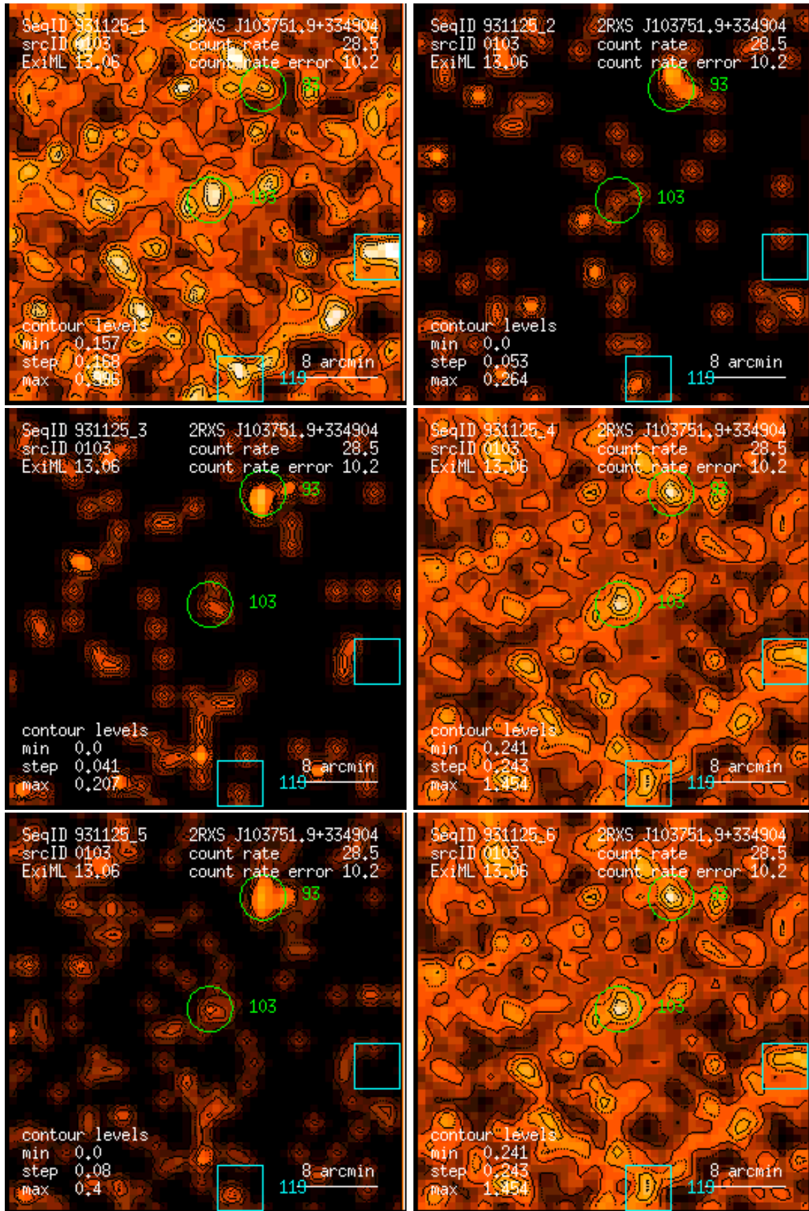
Figure 103: RASS 931125: detection 0103: band rate images, Gaussian filter: (1) PSPC channels 11 – 41, (2) 52 – 90, (3) 91 – 201, (4) 11 – 235, (5) 52 – 201, (6) 11 – 201. Broad band rates in counts/ks. Band rate contour levels in counts/ks/arcmin 2 .
