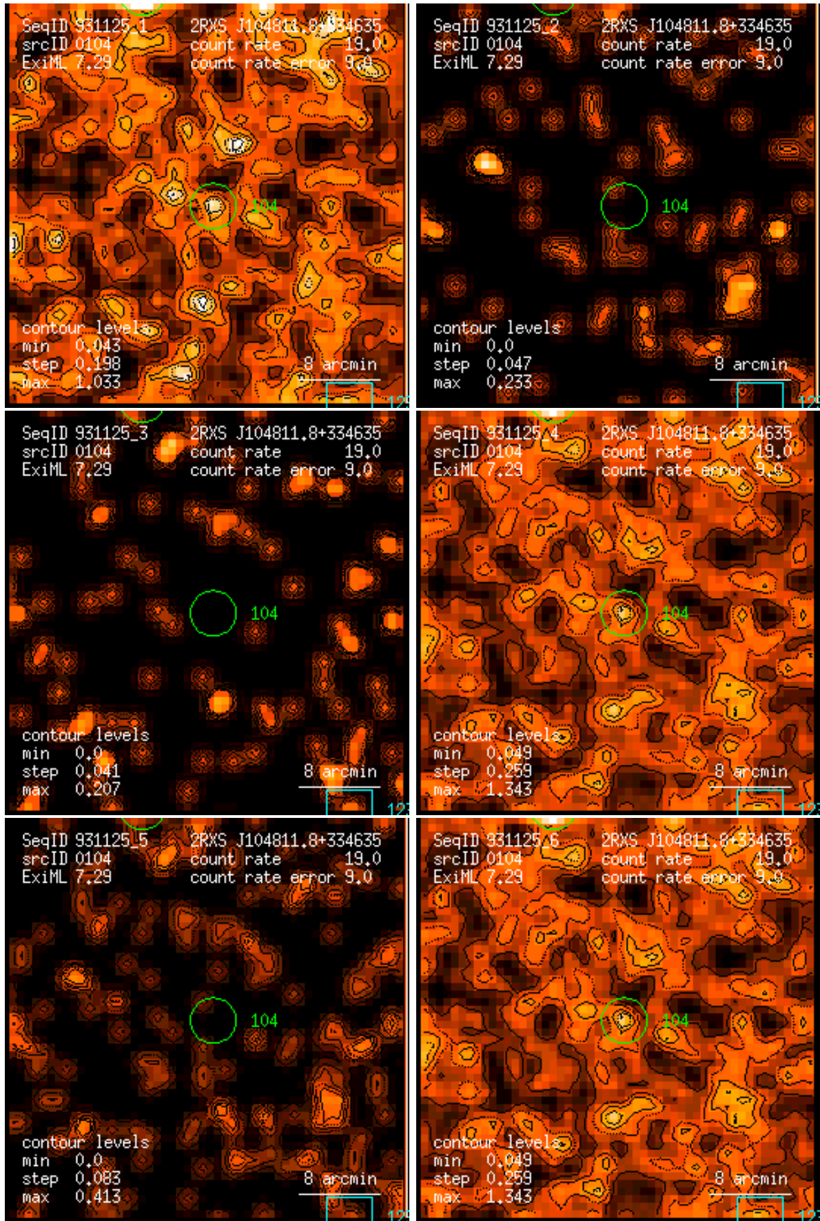
Figure 104: RASS 931125: detection 0104: band rate images, Gaussian filter: (1) PSPC channels 11 – 41, (2) 52 – 90, (3) 91 – 201, (4) 11 – 235, (5) 52 – 201, (6) 11 – 201. Broad band rates in counts/ks. Band rate contour levels in counts/ks/arcmin 2 .
