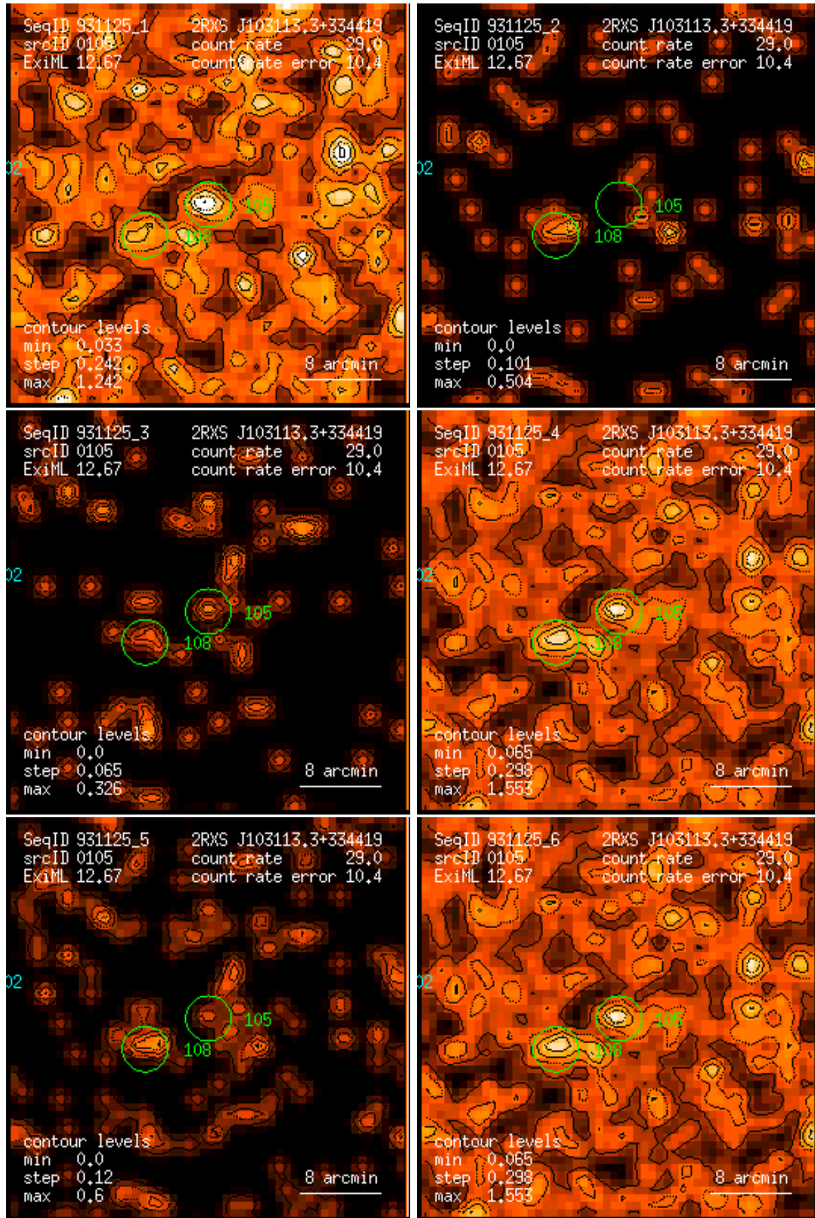
Figure 105: RASS 931125: detection 0105: band rate images, Gaussian filter: (1) PSPC channels 11 – 41, (2) 52 – 90, (3) 91 – 201, (4) 11 – 235, (5) 52 – 201, (6) 11 – 201. Broad band rates in counts/ks. Band rate contour levels in counts/ks/arcmin 2 .
