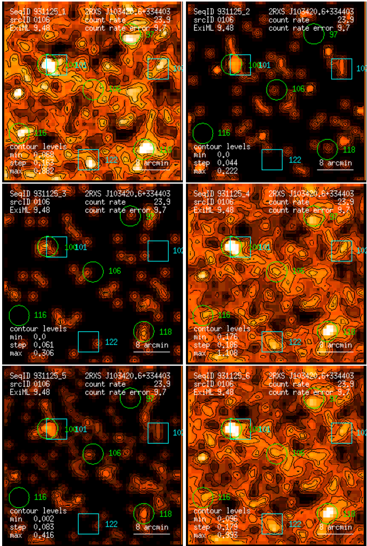
Figure 106: RASS 931125: detection 0106: band rate images, Gaussian filter: (1) PSPC channels 11 – 41, (2) 52 – 90, (3) 91 – 201, (4) 11 – 235, (5) 52 – 201, (6) 11 – 201. Broad band rates in counts/ks. Band rate contour levels in counts/ks/arcmin 2 .
