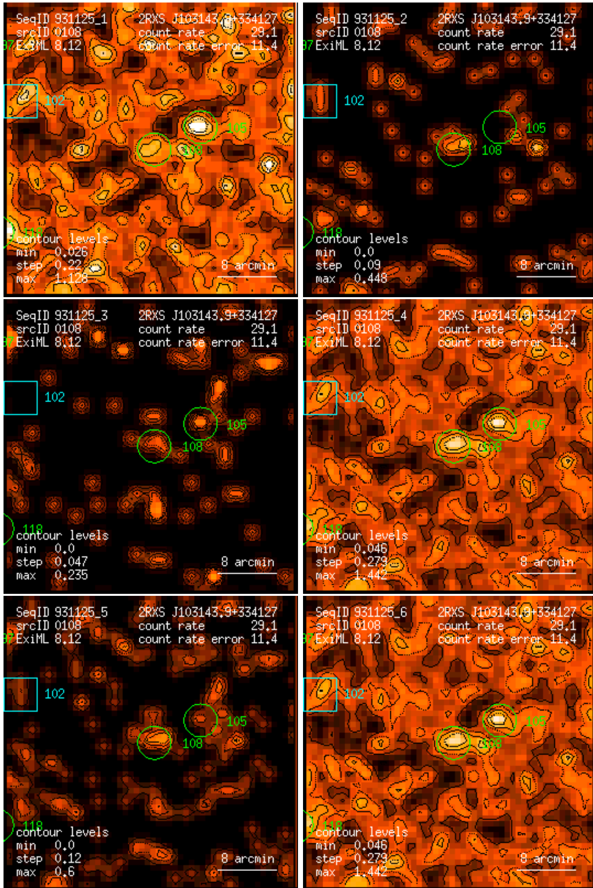
Figure 108: RASS 931125: detection 0108: band rate images, Gaussian filter: (1) PSPC channels 11 – 41, (2) 52 – 90, (3) 91 – 201, (4) 11 – 235, (5) 52 – 201, (6) 11 – 201. Broad band rates in counts/ks. Band rate contour levels in counts/ks/arcmin 2 .
