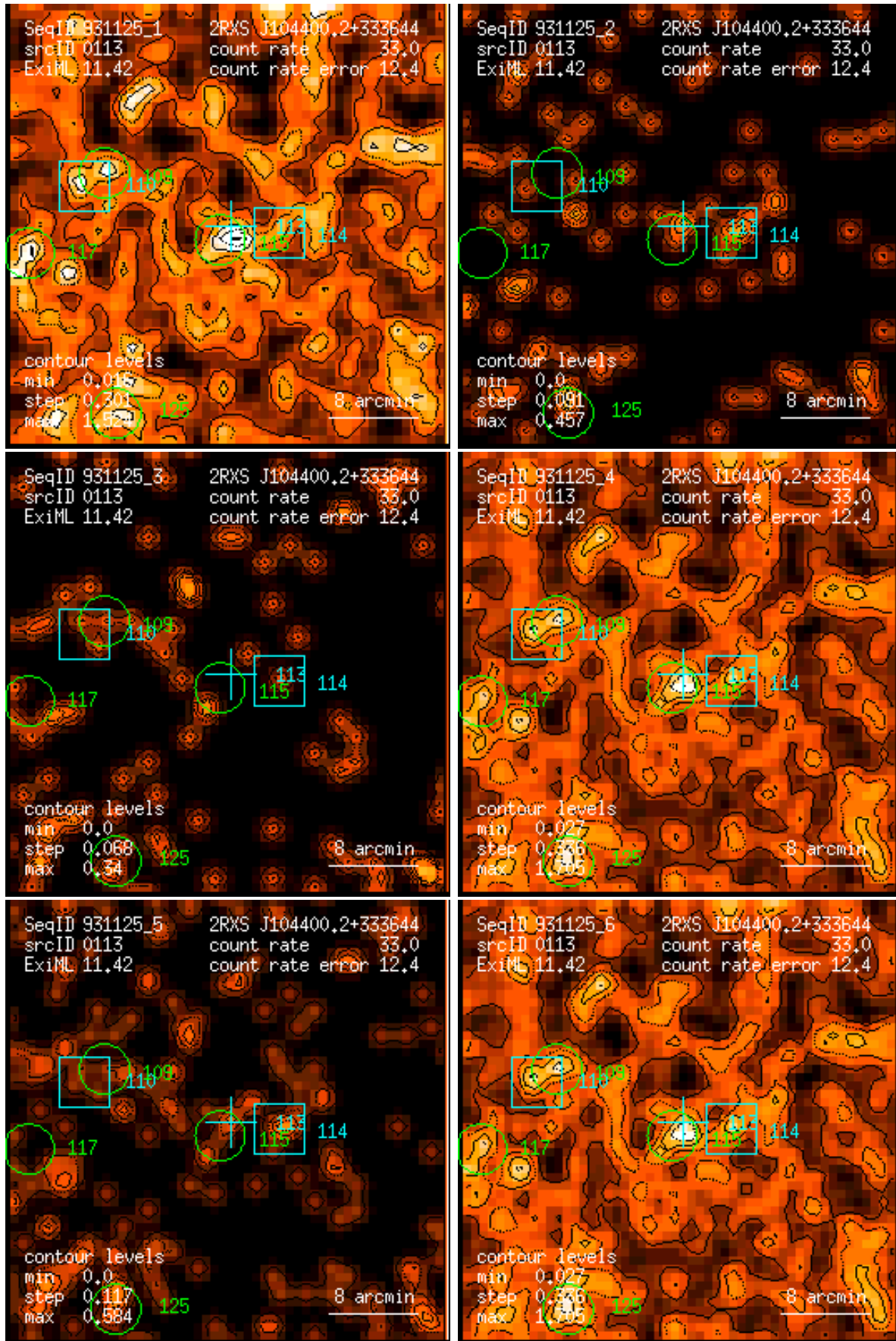
Figure 113: RASS 931125: detection 0113: band rate images, Gaussian filter: (1) PSPC channels 11 – 41, (2) 52 – 90, (3) 91 – 201, (4) 11 – 235, (5) 52 – 201, (6) 11 – 201. Broad band rates in counts/ks. Band rate contour levels in counts/ks/arcmin 2 .
