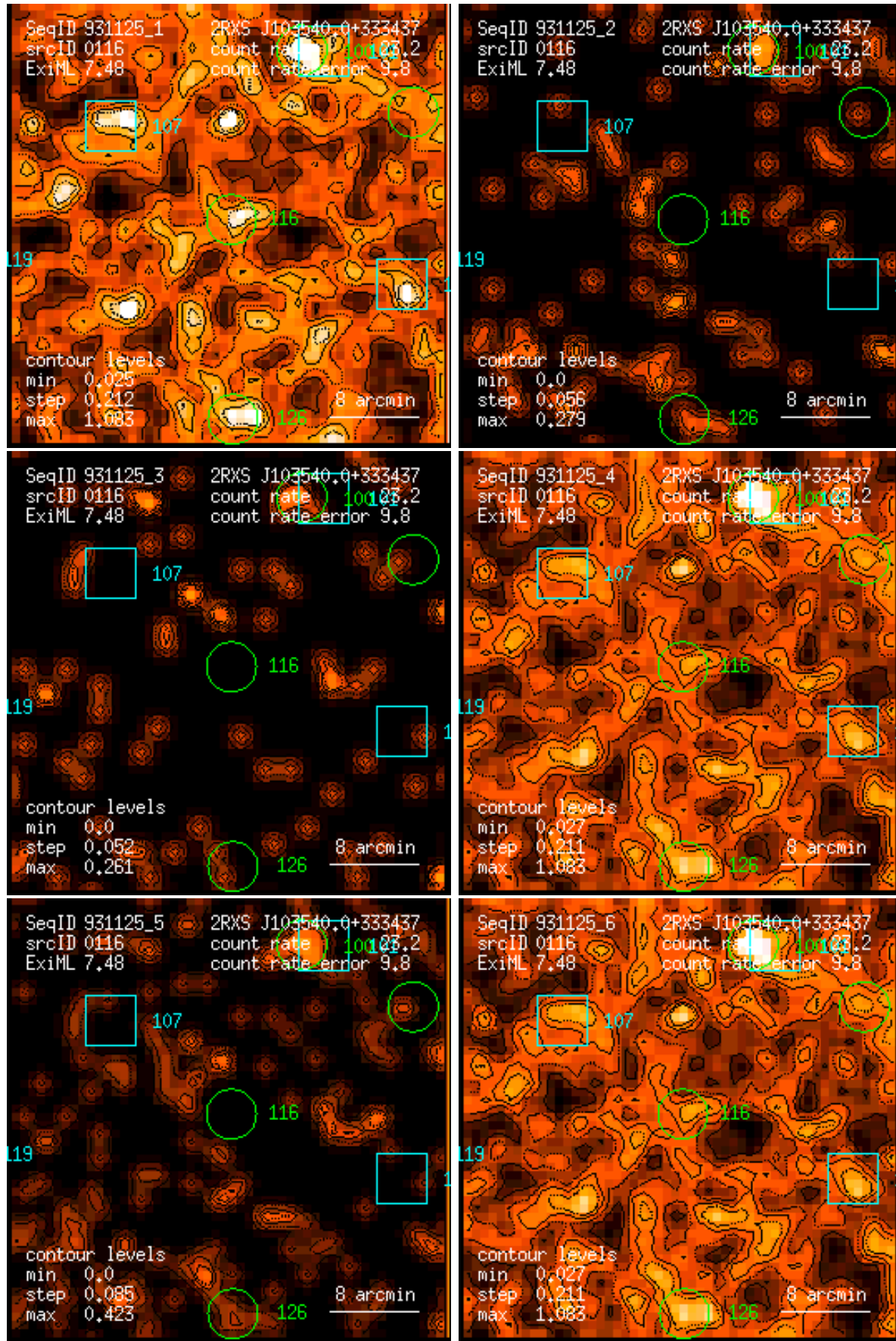
Figure 116: RASS 931125: detection 0116: band rate images, Gaussian filter: (1) PSPC channels 11 – 41, (2) 52 – 90, (3) 91 – 201, (4) 11 – 235, (5) 52 – 201, (6) 11 – 201. Broad band rates in counts/ks. Band rate contour levels in counts/ks/arcmin 2 .
