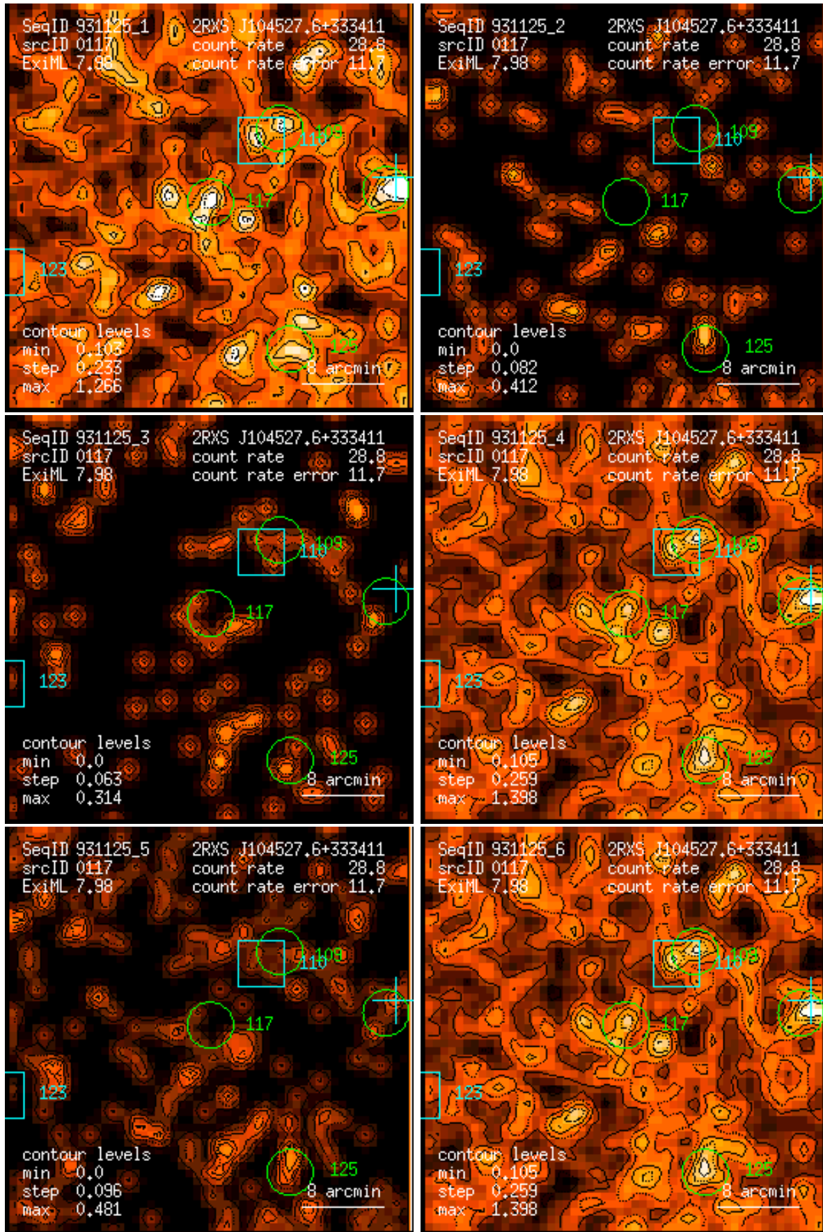
Figure 117: RASS 931125: detection 0117: band rate images, Gaussian filter: (1) PSPC channels 11 – 41, (2) 52 – 90, (3) 91 – 201, (4) 11 – 235, (5) 52 – 201, (6) 11 – 201. Broad band rates in counts/ks. Band rate contour levels in counts/ks/arcmin 2 .
