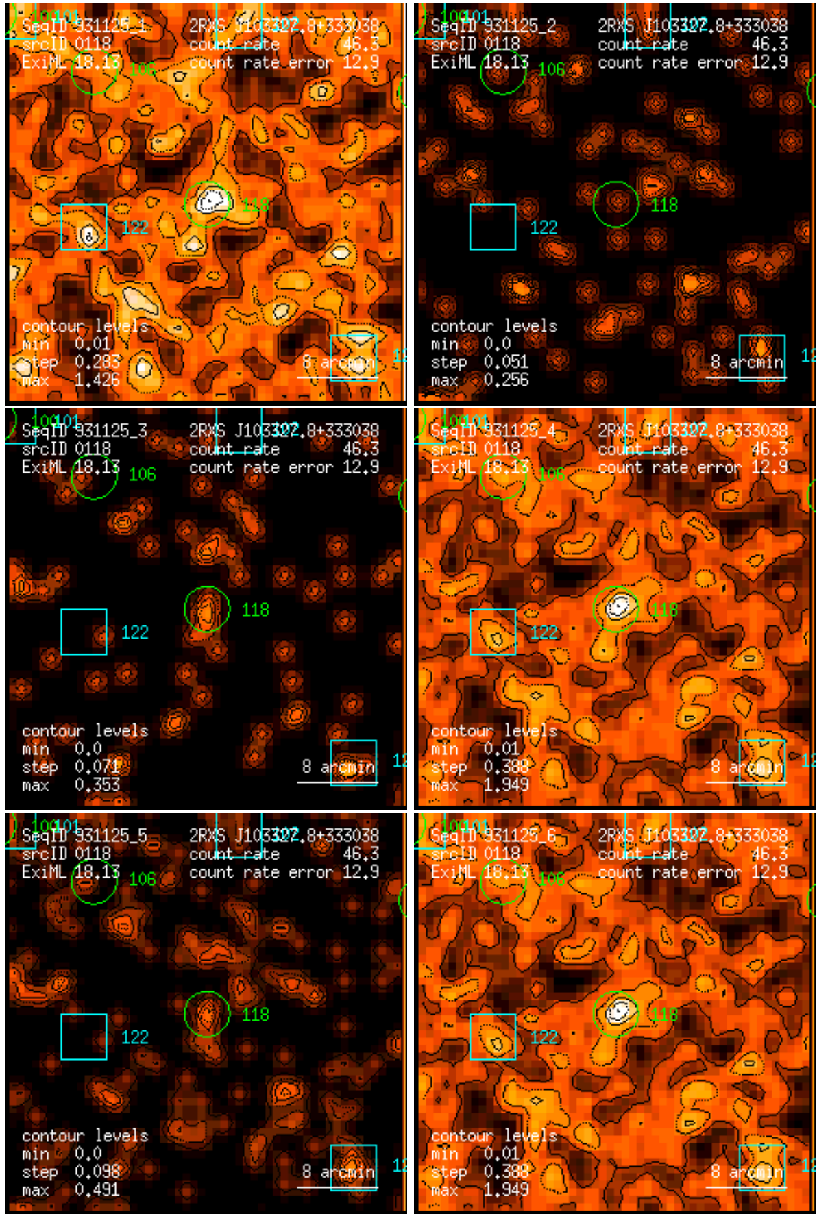
Figure 118: RASS 931125: detection 0118: band rate images, Gaussian filter: (1) PSPC channels 11 – 41, (2) 52 – 90, (3) 91 – 201, (4) 11 – 235, (5) 52 – 201, (6) 11 – 201. Broad band rates in counts/ks. Band rate contour levels in counts/ks/arcmin 2 .
