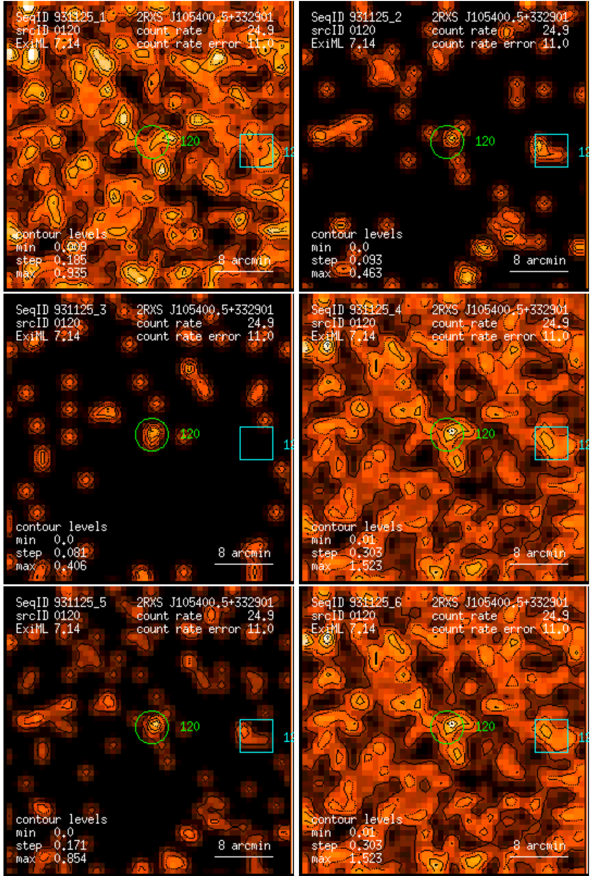
Figure 120: RASS 931125: detection 0120: band rate images, Gaussian filter: (1) PSPC channels 11 – 41, (2) 52 – 90, (3) 91 – 201, (4) 11 – 235, (5) 52 – 201, (6) 11 – 201. Broad band rates in counts/ks. Band rate contour levels in counts/ks/arcmin 2 .
