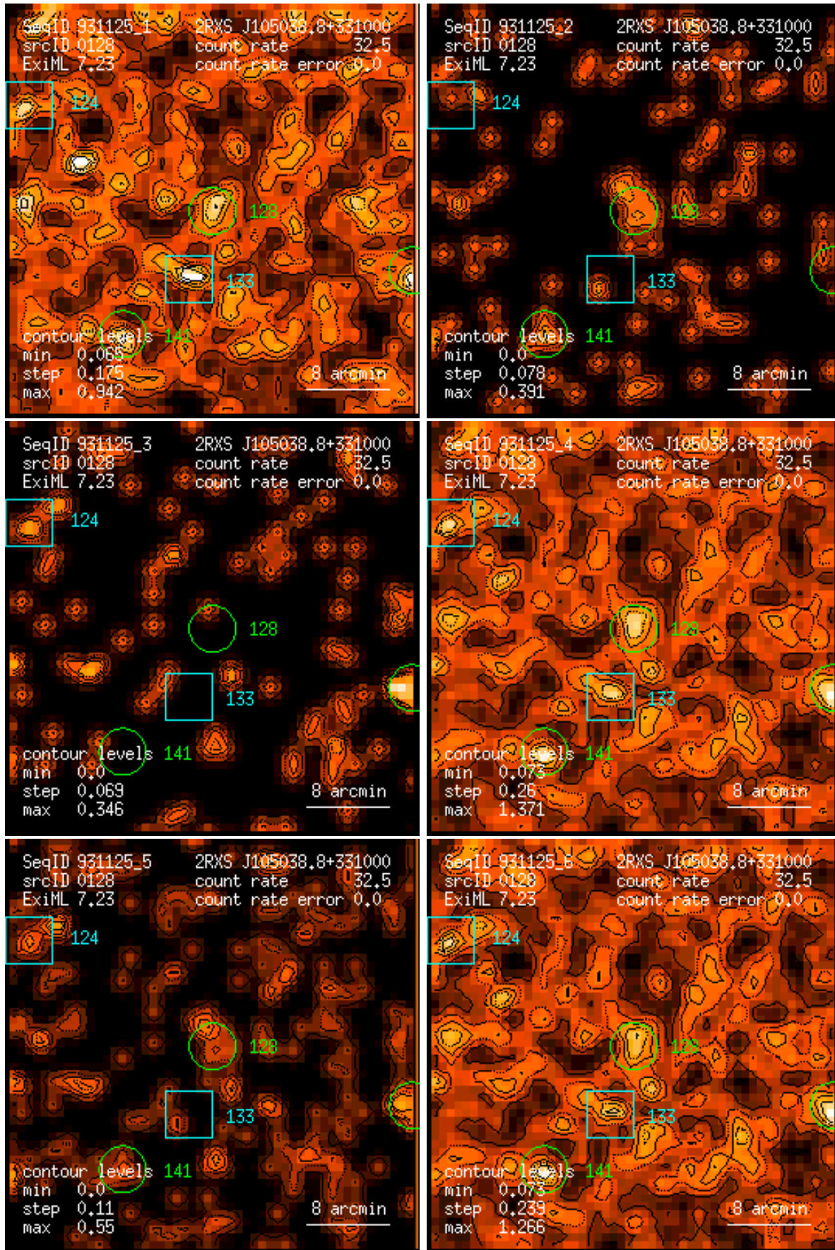
Figure 128: RASS 931125: detection 0128: band rate images, Gaussian filter: (1) PSPC channels 11 – 41, (2) 52 – 90, (3) 91 – 201, (4) 11 – 235, (5) 52 – 201, (6) 11 – 201. Broad band rates in counts/ks. Band rate contour levels in counts/ks/arcmin 2 .
