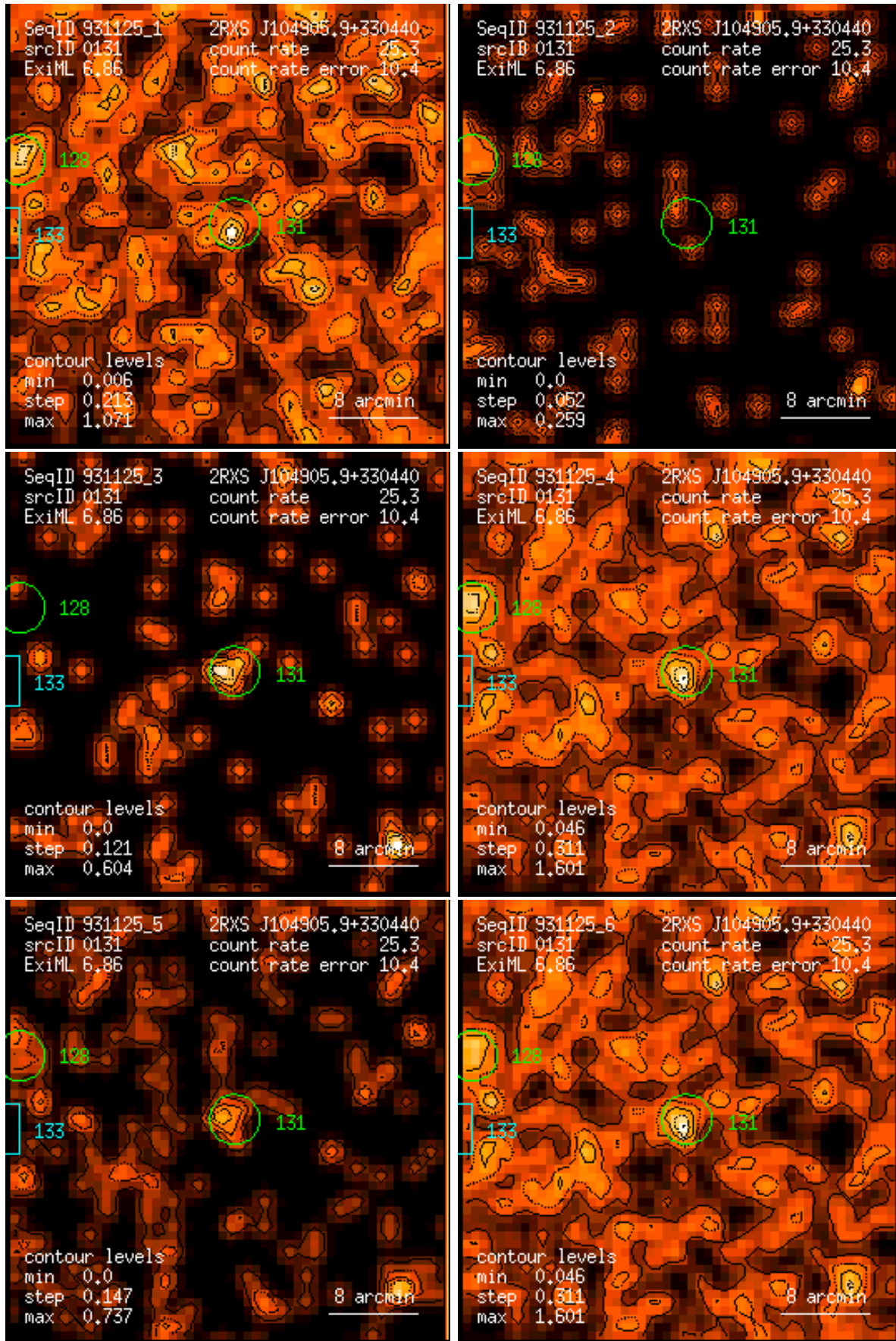
Figure 131: RASS 931125: detection 0131: band rate images, Gaussian filter: (1) PSPC channels 11 – 41, (2) 52 – 90, (3) 91 – 201, (4) 11 – 235, (5) 52 – 201, (6) 11 – 201. Broad band rates in counts/ks. Band rate contour levels in counts/ks/arcmin 2 .
