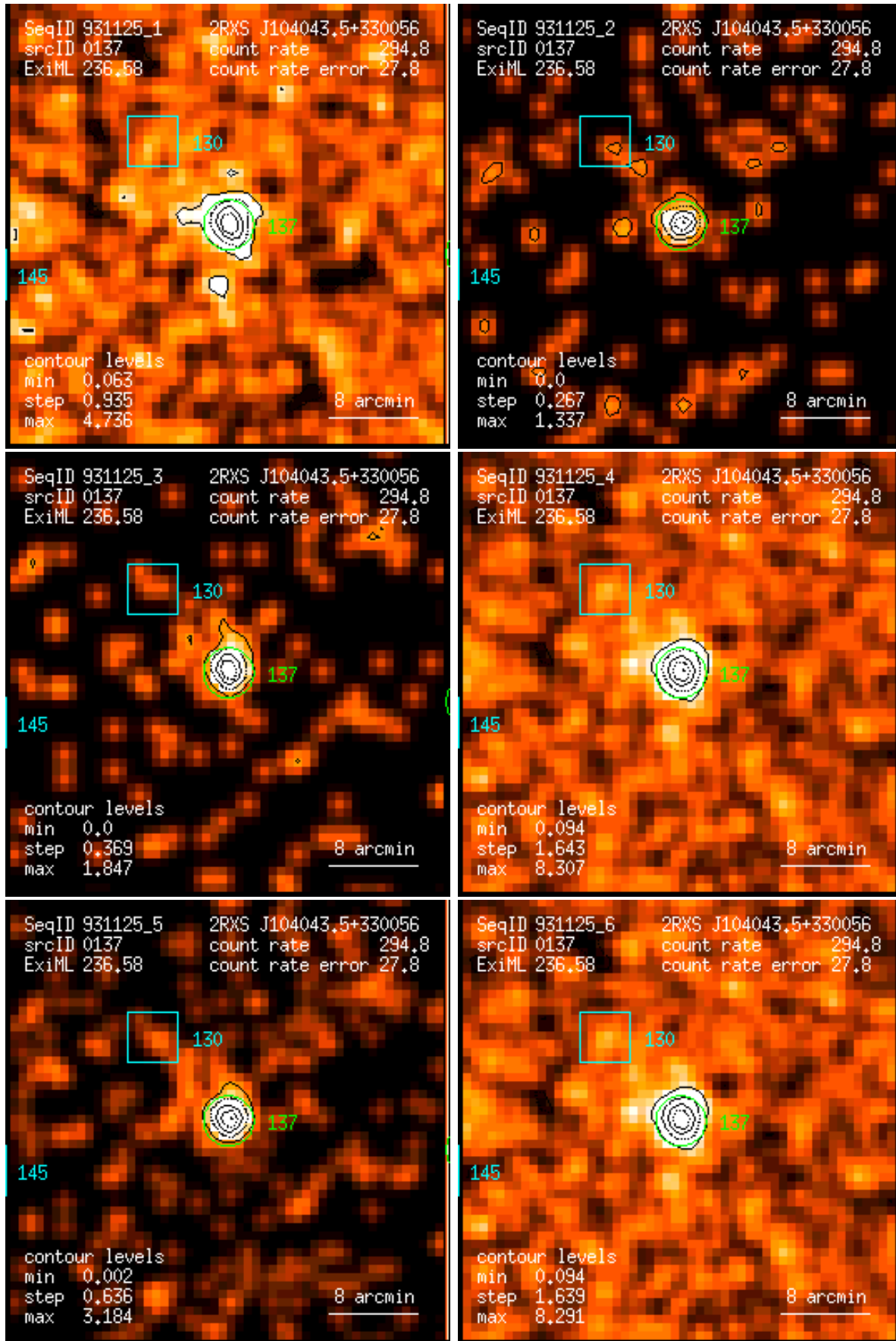
Figure 137: RASS 931125: detection 0137: band rate images, Gaussian filter: (1) PSPC channels 11 – 41, (2) 52 – 90, (3) 91 – 201, (4) 11 – 235, (5) 52 – 201, (6) 11 – 201. Broad band rates in counts/ks. Band rate contour levels in counts/ks/arcmin 2 .
