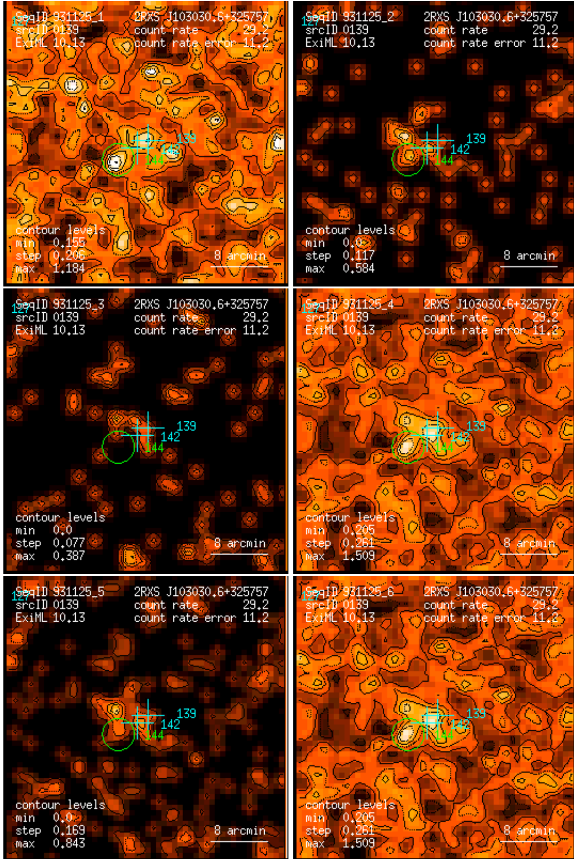
Figure 139: RASS 931125: detection 0139: band rate images, Gaussian filter: (1) PSPC channels 11 – 41, (2) 52 – 90, (3) 91 – 201, (4) 11 – 235, (5) 52 – 201, (6) 11 – 201. Broad band rates in counts/ks. Band rate contour levels in counts/ks/arcmin 2 .
