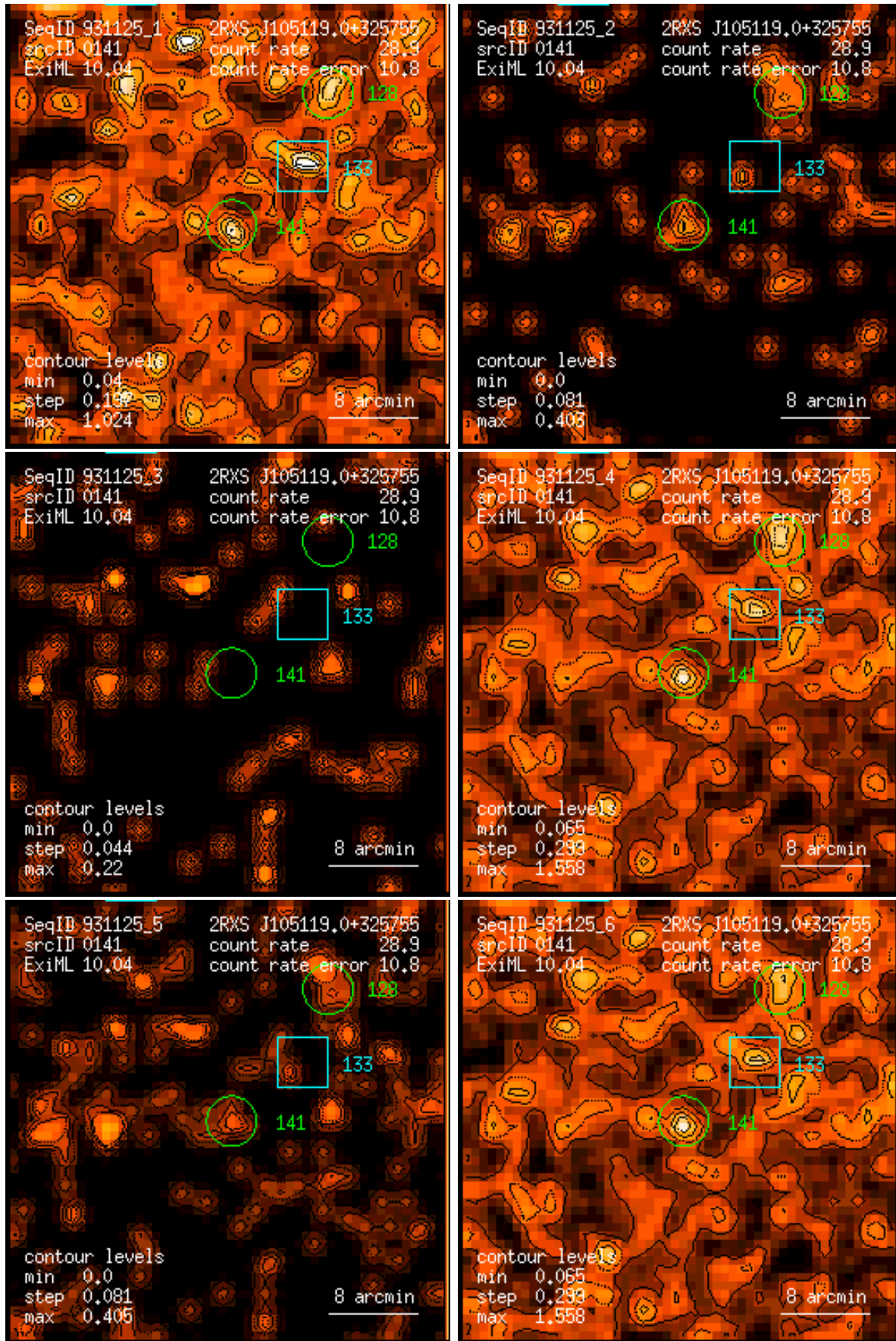
Figure 141: RASS 931125: detection 0141: band rate images, Gaussian filter: (1) PSPC channels 11 – 41, (2) 52 – 90, (3) 91 – 201, (4) 11 – 235, (5) 52 – 201, (6) 11 – 201. Broad band rates in counts/ks. Band rate contour levels in counts/ks/arcmin 2 .
