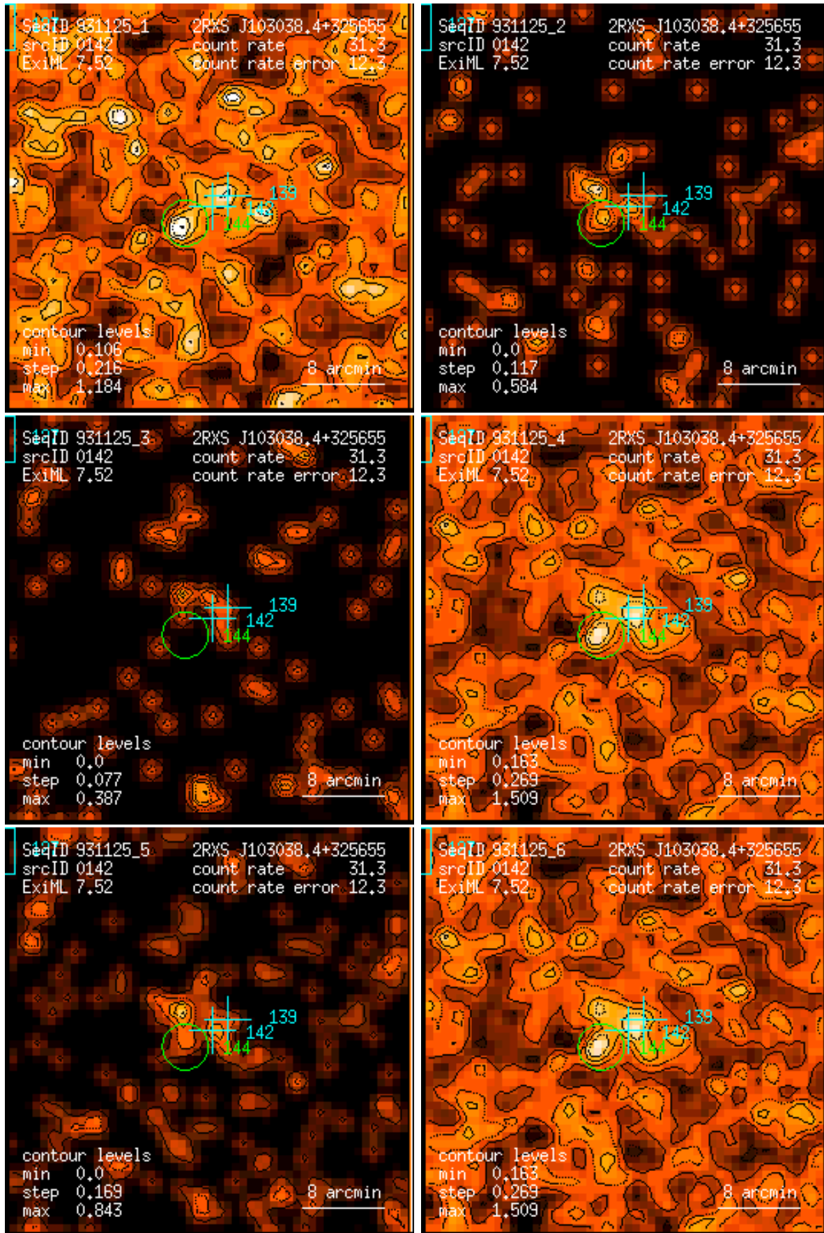
Figure 142: RASS 931125: detection 0142: band rate images, Gaussian filter: (1) PSPC channels 11 – 41, (2) 52 – 90, (3) 91 – 201, (4) 11 – 235, (5) 52 – 201, (6) 11 – 201. Broad band rates in counts/ks. Band rate contour levels in counts/ks/arcmin 2 .
