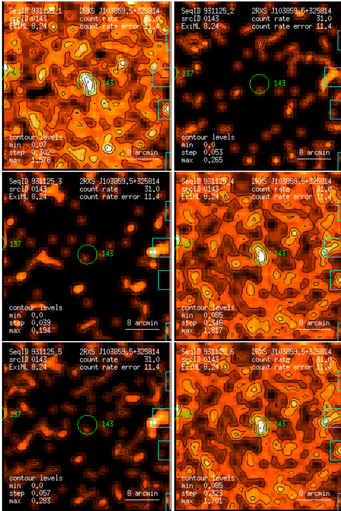
Figure 143: RASS 931125: detection 0143: band rate images, Gaussian filter: (1) PSPC channels 11 – 41, (2) 52 – 90, (3) 91 – 201, (4) 11 – 235, (5) 52 – 201, (6) 11 – 201. Broad band rates in counts/ks. Band rate contour levels in counts/ks/arcmin 2 .
