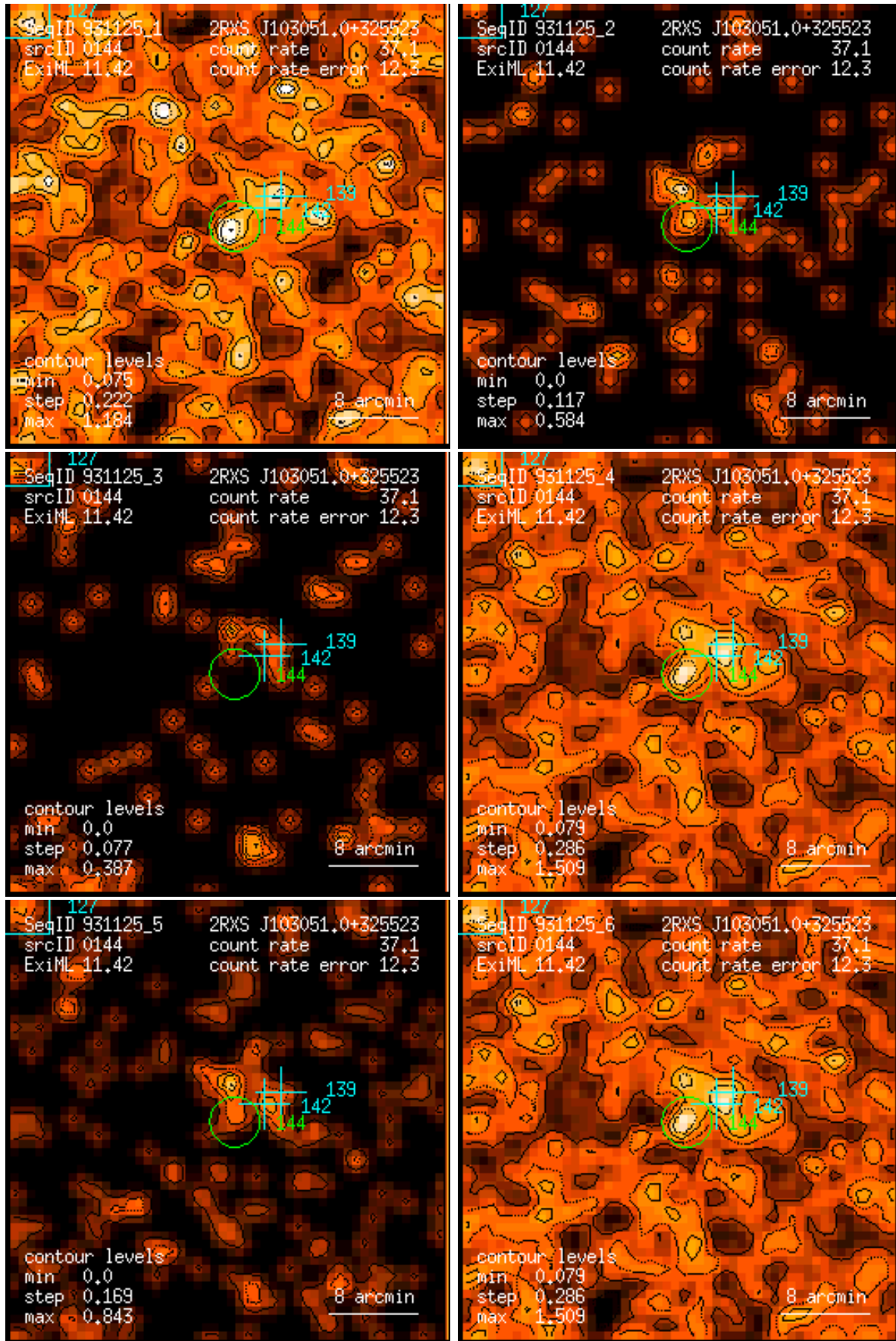
Figure 144: RASS 931125: detection 0144: band rate images, Gaussian filter: (1) PSPC channels 11 – 41, (2) 52 – 90, (3) 91 – 201, (4) 11 – 235, (5) 52 – 201, (6) 11 – 201. Broad band rates in counts/ks. Band rate contour levels in counts/ks/arcmin 2 .
