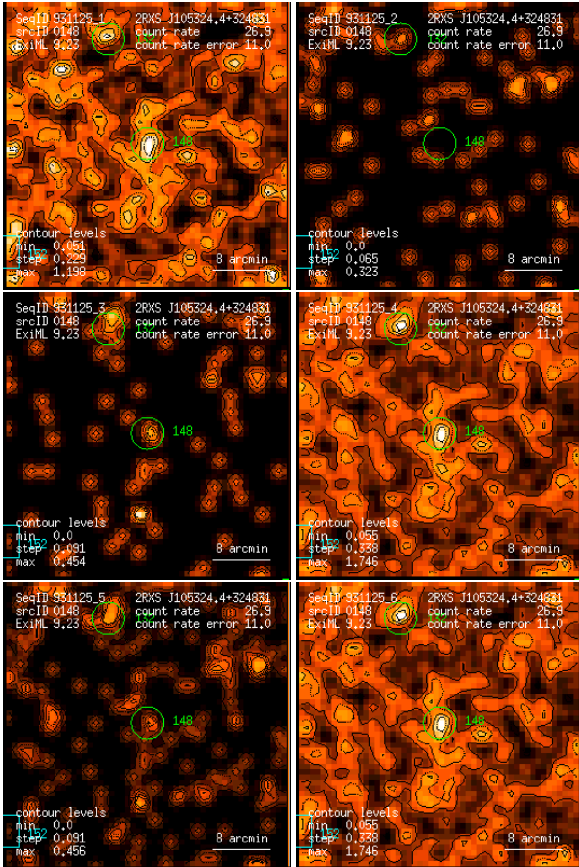
Figure 148: RASS 931125: detection 0148: band rate images, Gaussian filter: (1) PSPC channels 11 – 41, (2) 52 – 90, (3) 91 – 201, (4) 11 – 235, (5) 52 – 201, (6) 11 – 201. Broad band rates in counts/ks. Band rate contour levels in counts/ks/arcmin 2 .
