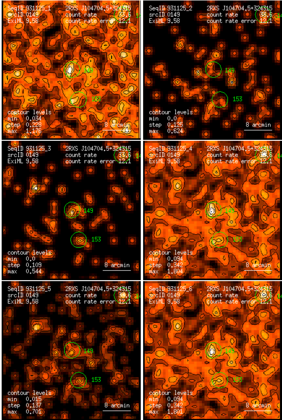
Figure 149: RASS 931125: detection 0149: band rate images, Gaussian filter: (1) PSPC channels 11 – 41, (2) 52 – 90, (3) 91 – 201, (4) 11 – 235, (5) 52 – 201, (6) 11 – 201. Broad band rates in counts/ks. Band rate contour levels in counts/ks/arcmin 2 .
