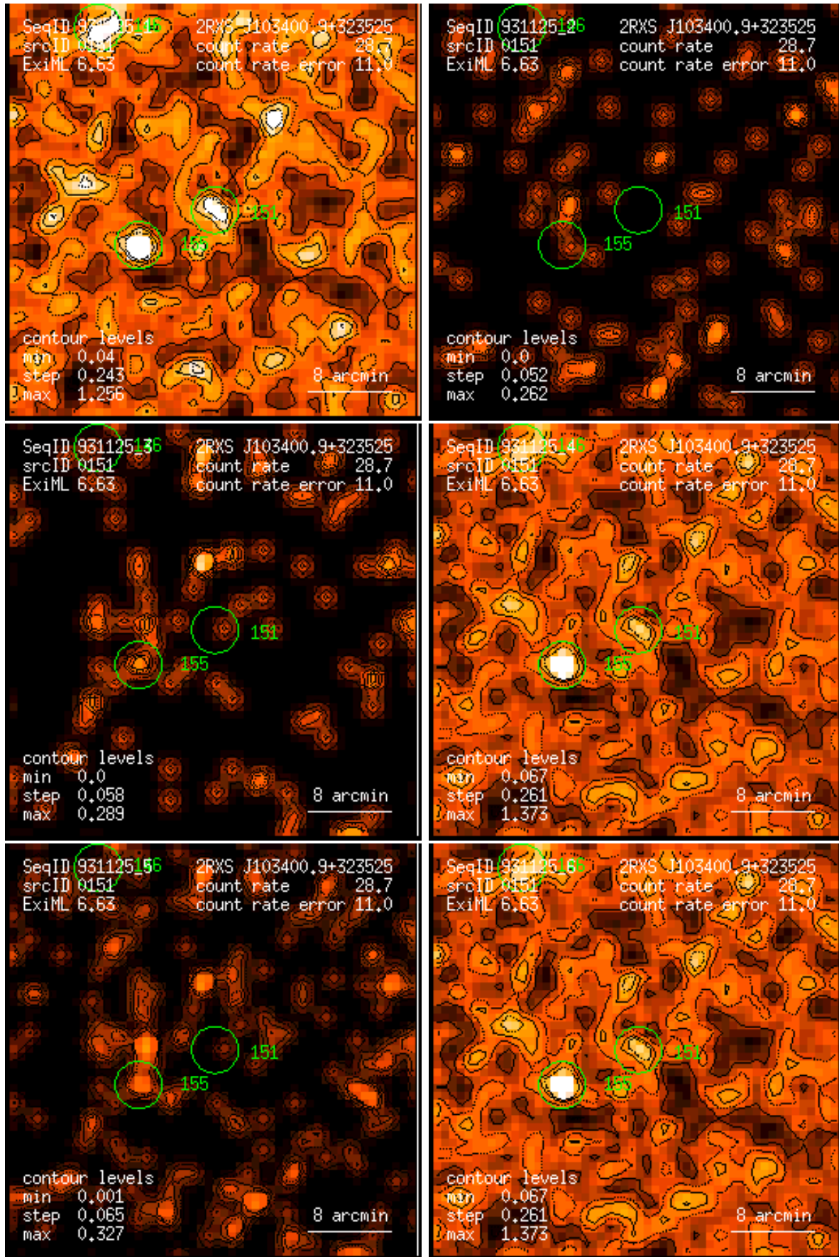
Figure 151: RASS 931125: detection 0151: band rate images, Gaussian filter: (1) PSPC channels 11 – 41, (2) 52 – 90, (3) 91 – 201, (4) 11 – 235, (5) 52 – 201, (6) 11 – 201. Broad band rates in counts/ks. Band rate contour levels in counts/ks/arcmin 2 .
