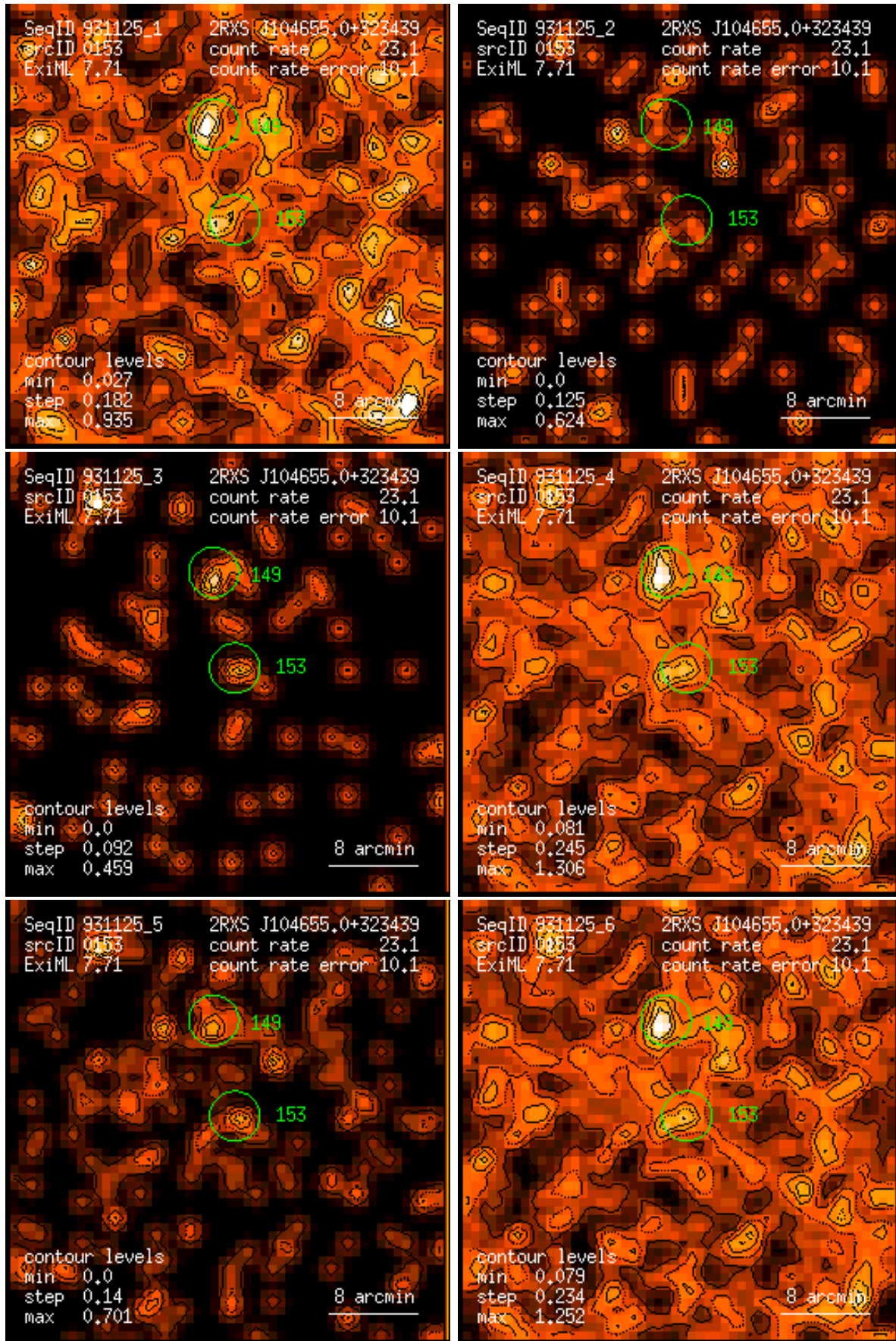
Figure 153: RASS 931125: detection 0153: band rate images, Gaussian filter: (1) PSPC channels 11 – 41, (2) 52 – 90, (3) 91 – 201, (4) 11 – 235, (5) 52 – 201, (6) 11 – 201. Broad band rates in counts/ks. Band rate contour levels in counts/ks/arcmin 2 .
