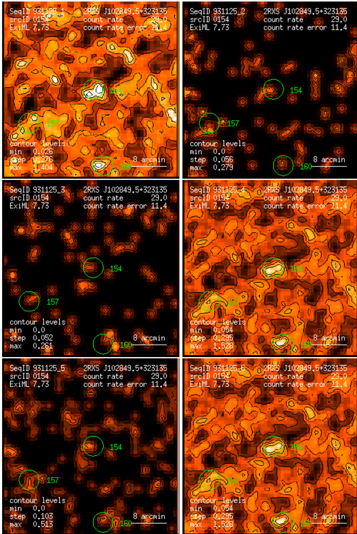
Figure 154: RASS 931125: detection 0154: band rate images, Gaussian filter: (1) PSPC channels 11 – 41, (2) 52 – 90, (3) 91 – 201, (4) 11 – 235, (5) 52 – 201, (6) 11 – 201. Broad band rates in counts/ks. Band rate contour levels in counts/ks/arcmin 2 .
