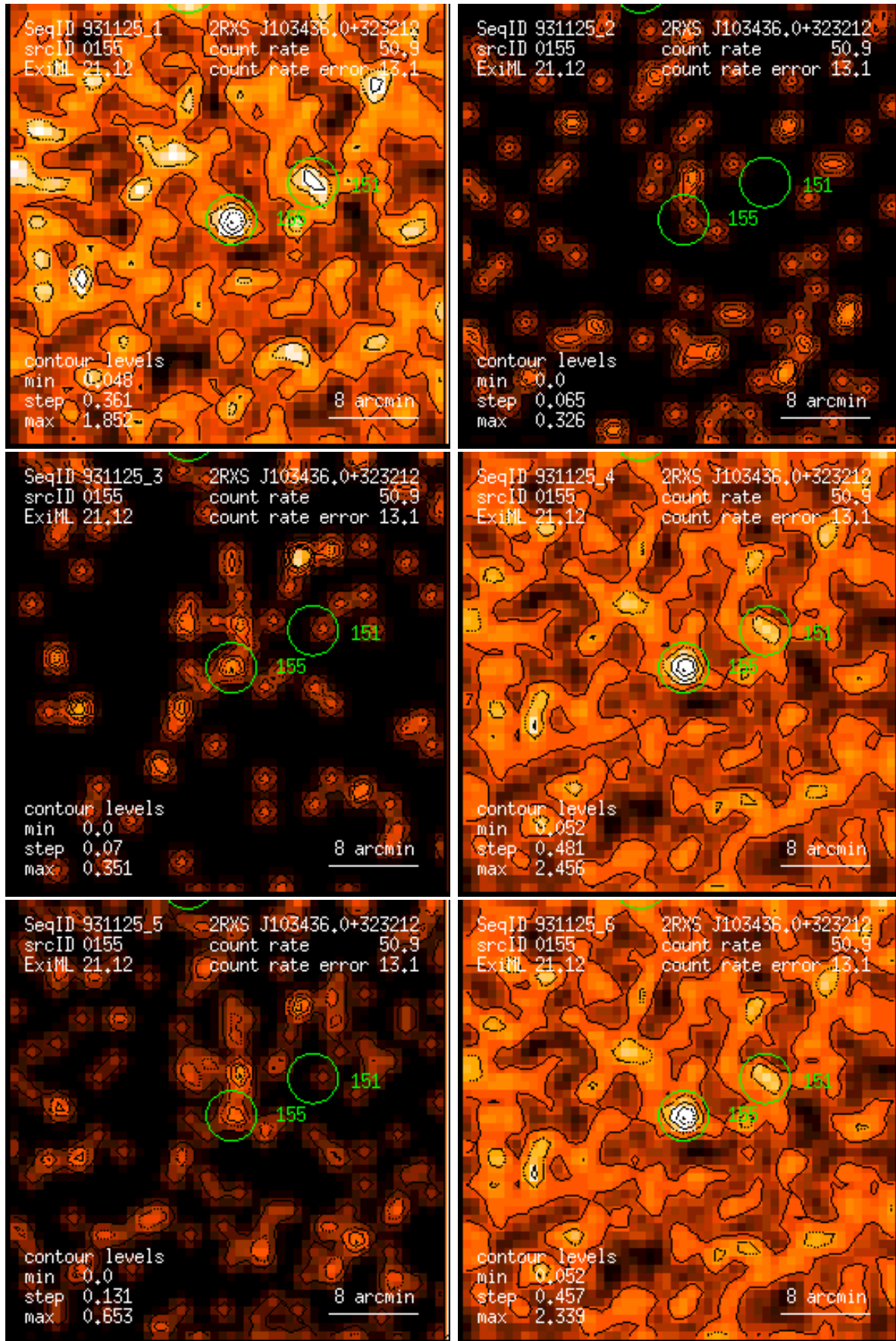
Figure 155: RASS 931125: detection 0155: band rate images, Gaussian filter: (1) PSPC channels 11 – 41, (2) 52 – 90, (3) 91 – 201, (4) 11 – 235, (5) 52 – 201, (6) 11 – 201. Broad band rates in counts/ks. Band rate contour levels in counts/ks/arcmin 2 .
