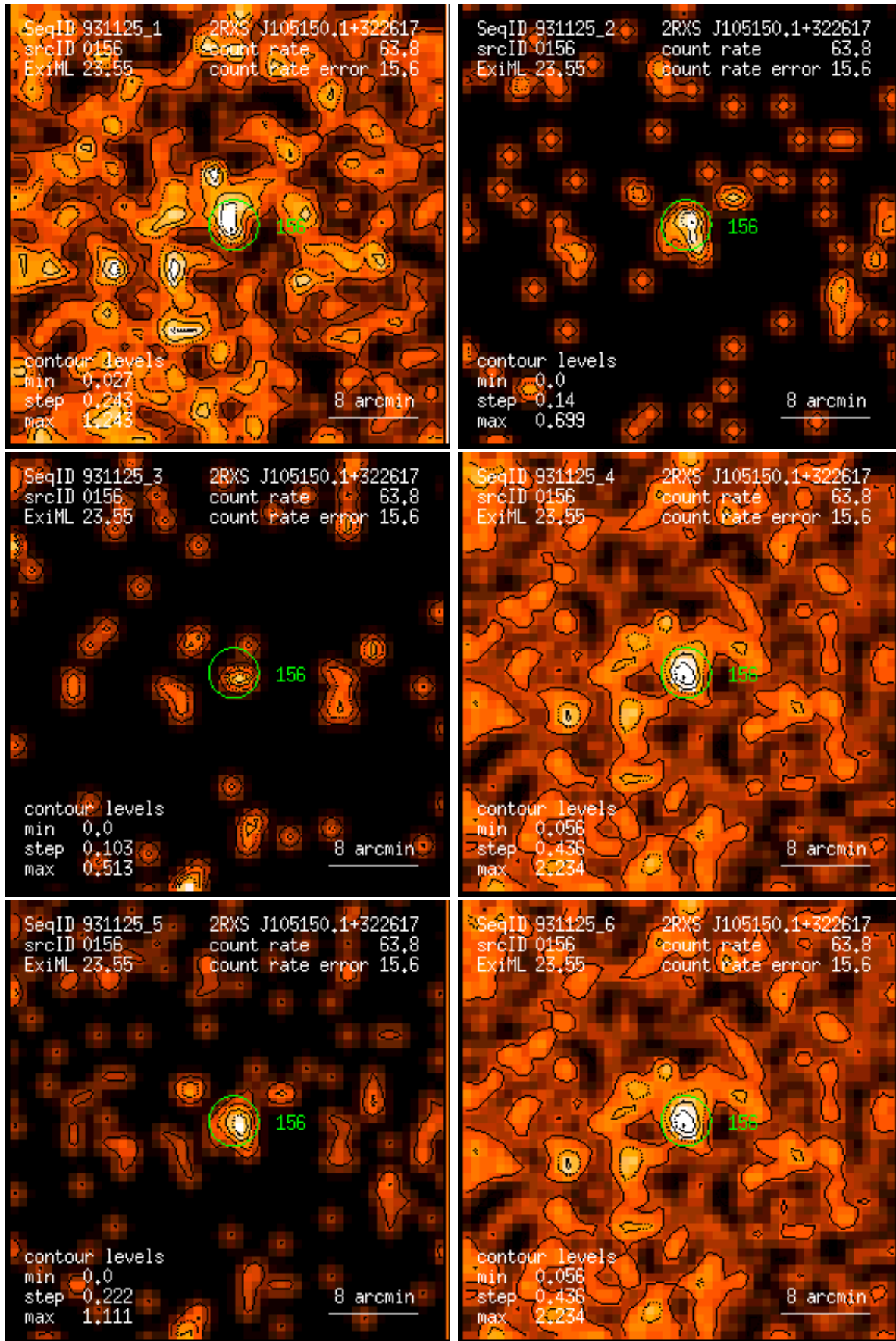
Figure 156: RASS 931125: detection 0156: band rate images, Gaussian filter: (1) PSPC channels 11 – 41, (2) 52 – 90, (3) 91 – 201, (4) 11 – 235, (5) 52 – 201, (6) 11 – 201. Broad band rates in counts/ks. Band rate contour levels in counts/ks/arcmin 2 .
