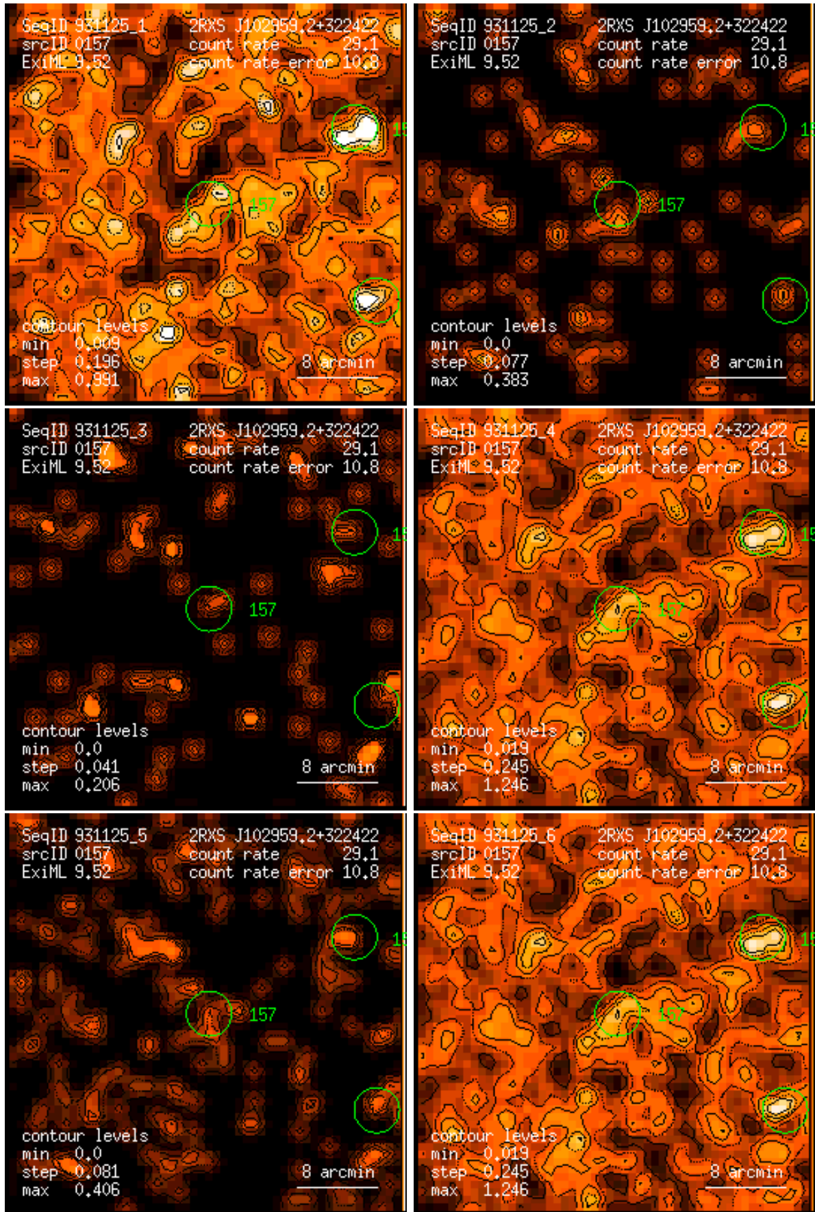
Figure 157: RASS 931125: detection 0157: band rate images, Gaussian filter: (1) PSPC channels 11 – 41, (2) 52 – 90, (3) 91 – 201, (4) 11 – 235, (5) 52 – 201, (6) 11 – 201. Broad band rates in counts/ks. Band rate contour levels in counts/ks/arcmin 2 .
