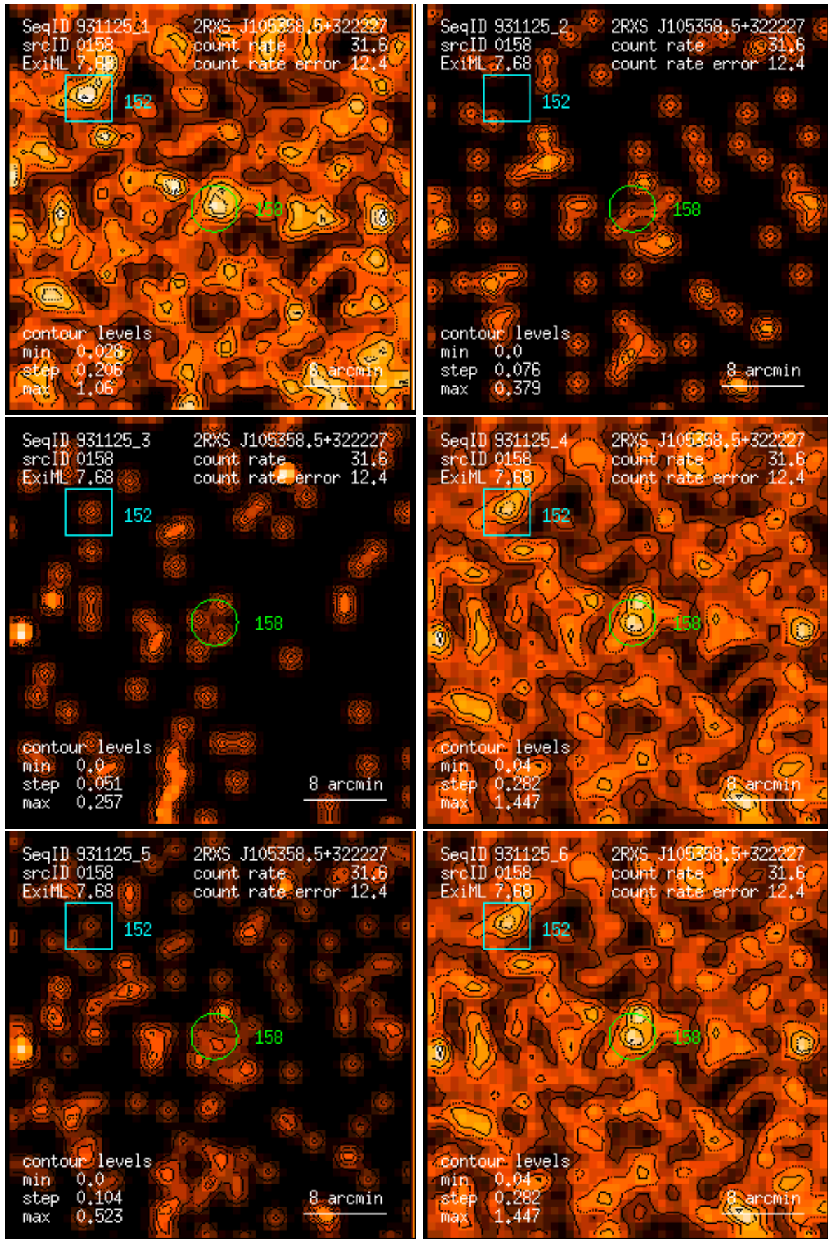
Figure 158: RASS 931125: detection 0158: band rate images, Gaussian filter: (1) PSPC channels 11 – 41, (2) 52 – 90, (3) 91 – 201, (4) 11 – 235, (5) 52 – 201, (6) 11 – 201. Broad band rates in counts/ks. Band rate contour levels in counts/ks/arcmin 2 .
