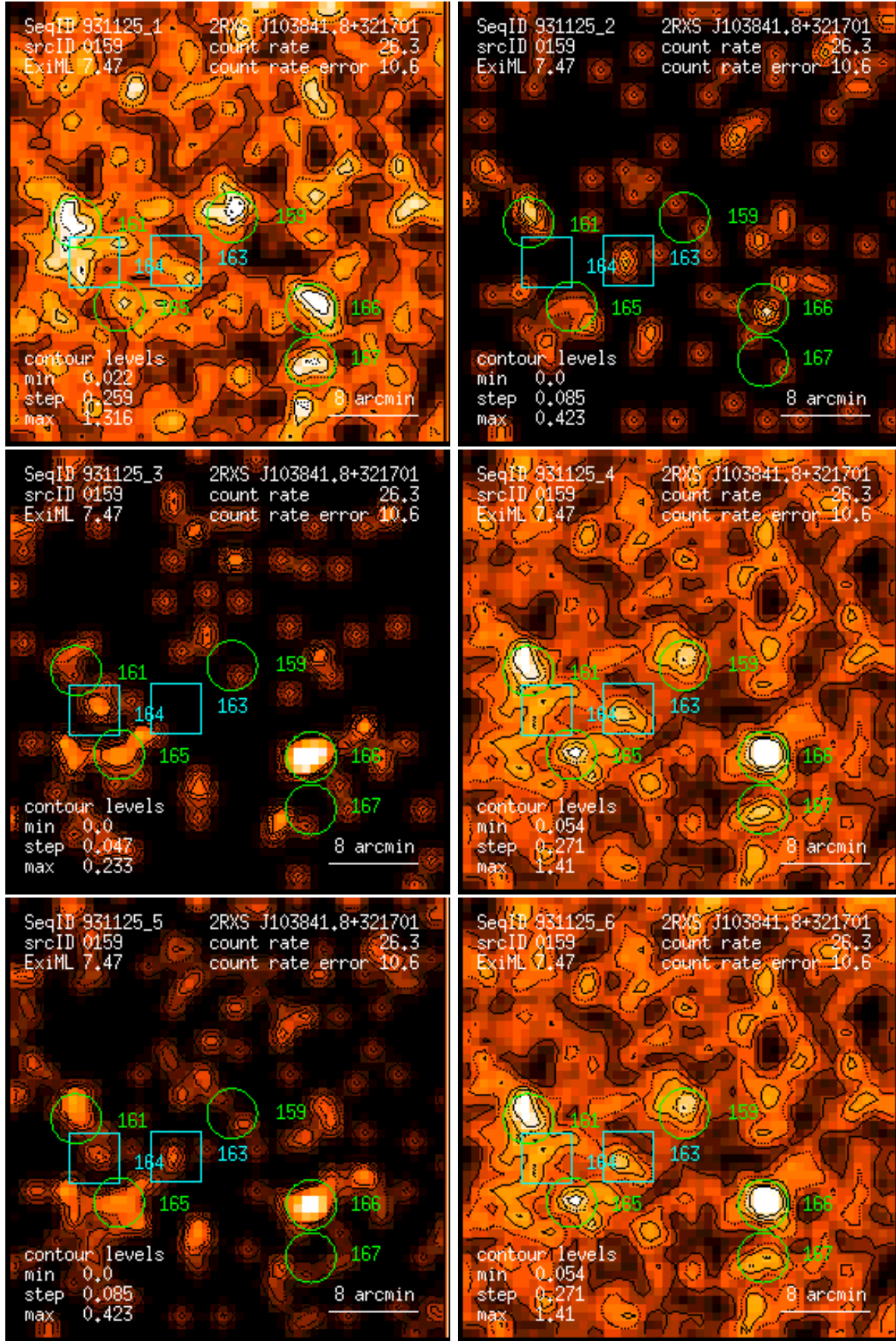
Figure 159: RASS 931125: detection 0159: band rate images, Gaussian filter: (1) PSPC channels 11 – 41, (2) 52 – 90, (3) 91 – 201, (4) 11 – 235, (5) 52 – 201, (6) 11 – 201. Broad band rates in counts/ks. Band rate contour levels in counts/ks/arcmin 2 .
