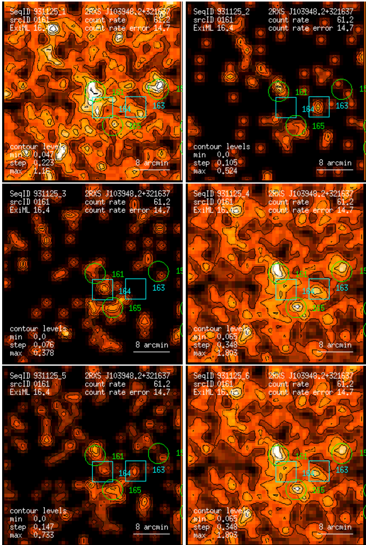
Figure 161: RASS 931125: detection 0161: band rate images, Gaussian filter: (1) PSPC channels 11 – 41, (2) 52 – 90, (3) 91 – 201, (4) 11 – 235, (5) 52 – 201, (6) 11 – 201. Broad band rates in counts/ks. Band rate contour levels in counts/ks/arcmin 2 .
