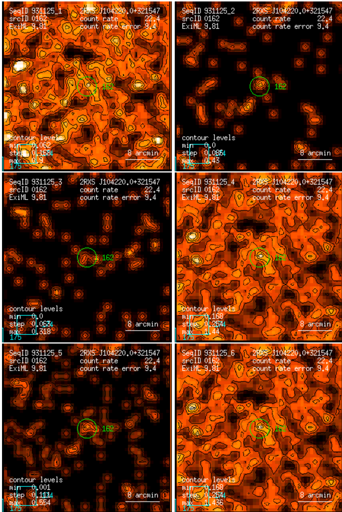
Figure 162: RASS 931125: detection 0162: band rate images, Gaussian filter: (1) PSPC channels 11 – 41, (2) 52 – 90, (3) 91 – 201, (4) 11 – 235, (5) 52 – 201, (6) 11 – 201. Broad band rates in counts/ks. Band rate contour levels in counts/ks/arcmin 2 .
