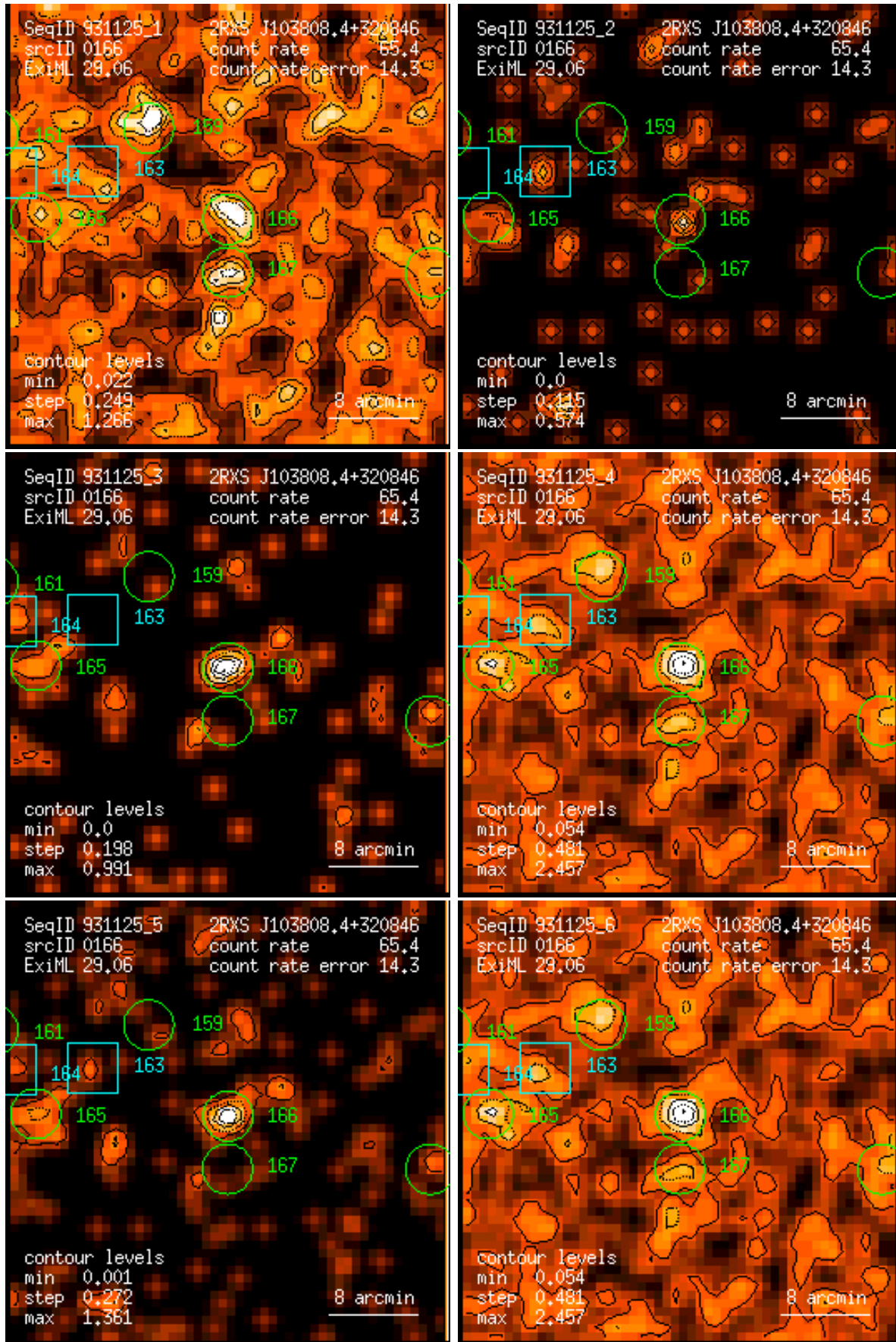
Figure 166: RASS 931125: detection 0166: band rate images, Gaussian filter: (1) PSPC channels 11 – 41, (2) 52 – 90, (3) 91 – 201, (4) 11 – 235, (5) 52 – 201, (6) 11 – 201. Broad band rates in counts/ks. Band rate contour levels in counts/ks/arcmin 2 .
