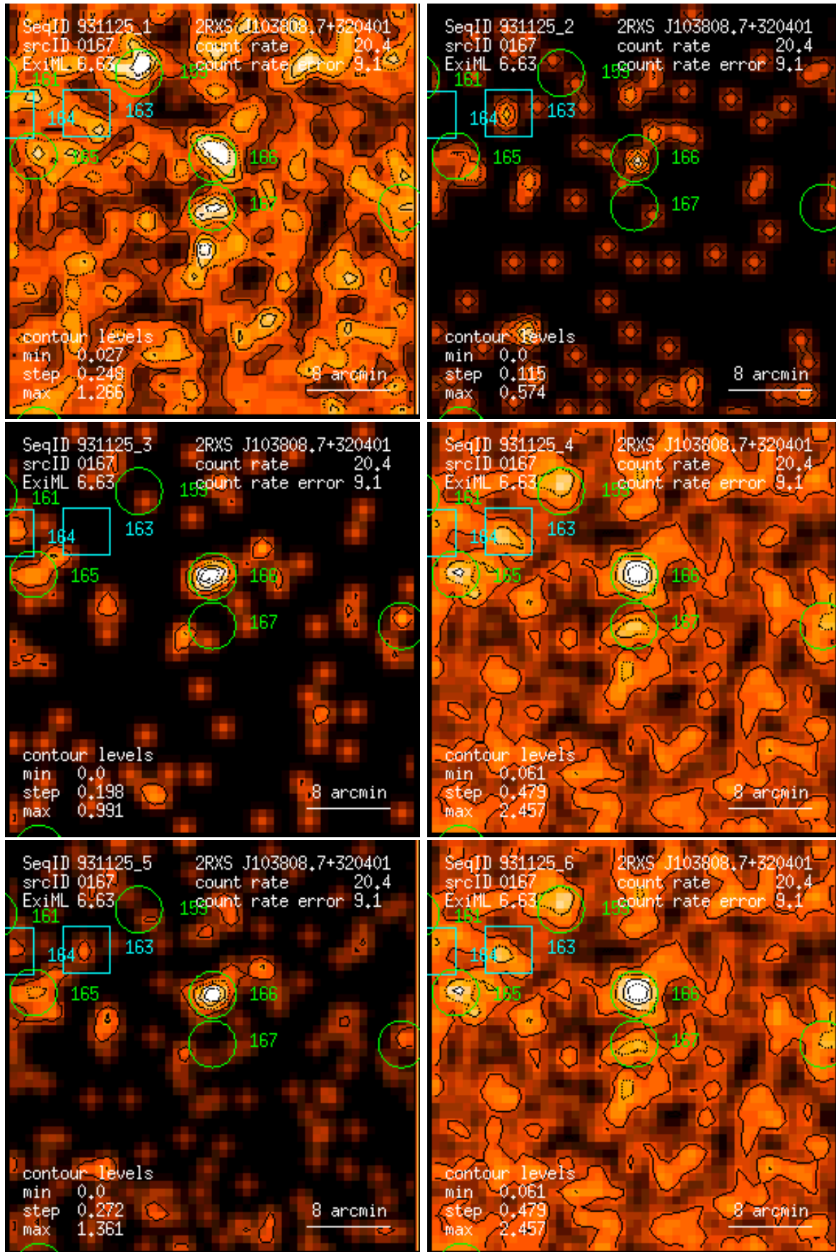
Figure 167: RASS 931125: detection 0167: band rate images, Gaussian filter: (1) PSPC channels 11 – 41, (2) 52 – 90, (3) 91 – 201, (4) 11 – 235, (5) 52 – 201, (6) 11 – 201. Broad band rates in counts/ks. Band rate contour levels in counts/ks/arcmin 2 .
