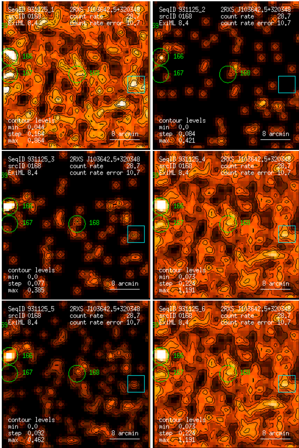
Figure 168: RASS 931125: detection 0168: band rate images, Gaussian filter: (1) PSPC channels 11 – 41, (2) 52 – 90, (3) 91 – 201, (4) 11 – 235, (5) 52 – 201, (6) 11 – 201. Broad band rates in counts/ks. Band rate contour levels in counts/ks/arcmin 2 .
