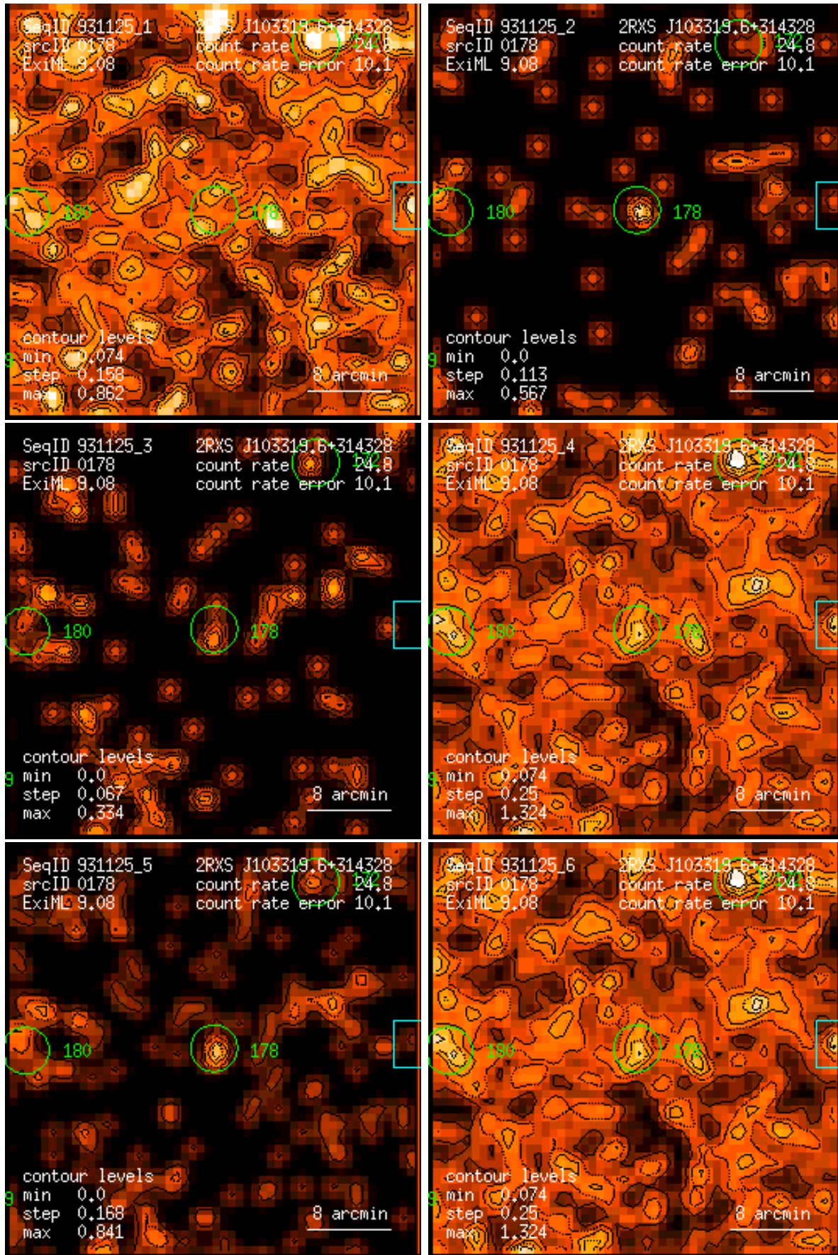
Figure 178: RASS 931125: detection 0178: band rate images, Gaussian filter: (1) PSPC channels 11 – 41, (2) 52 – 90, (3) 91 – 201, (4) 11 – 235, (5) 52 – 201, (6) 11 – 201. Broad band rates in counts/ks. Band rate contour levels in counts/ks/arcmin 2 .
