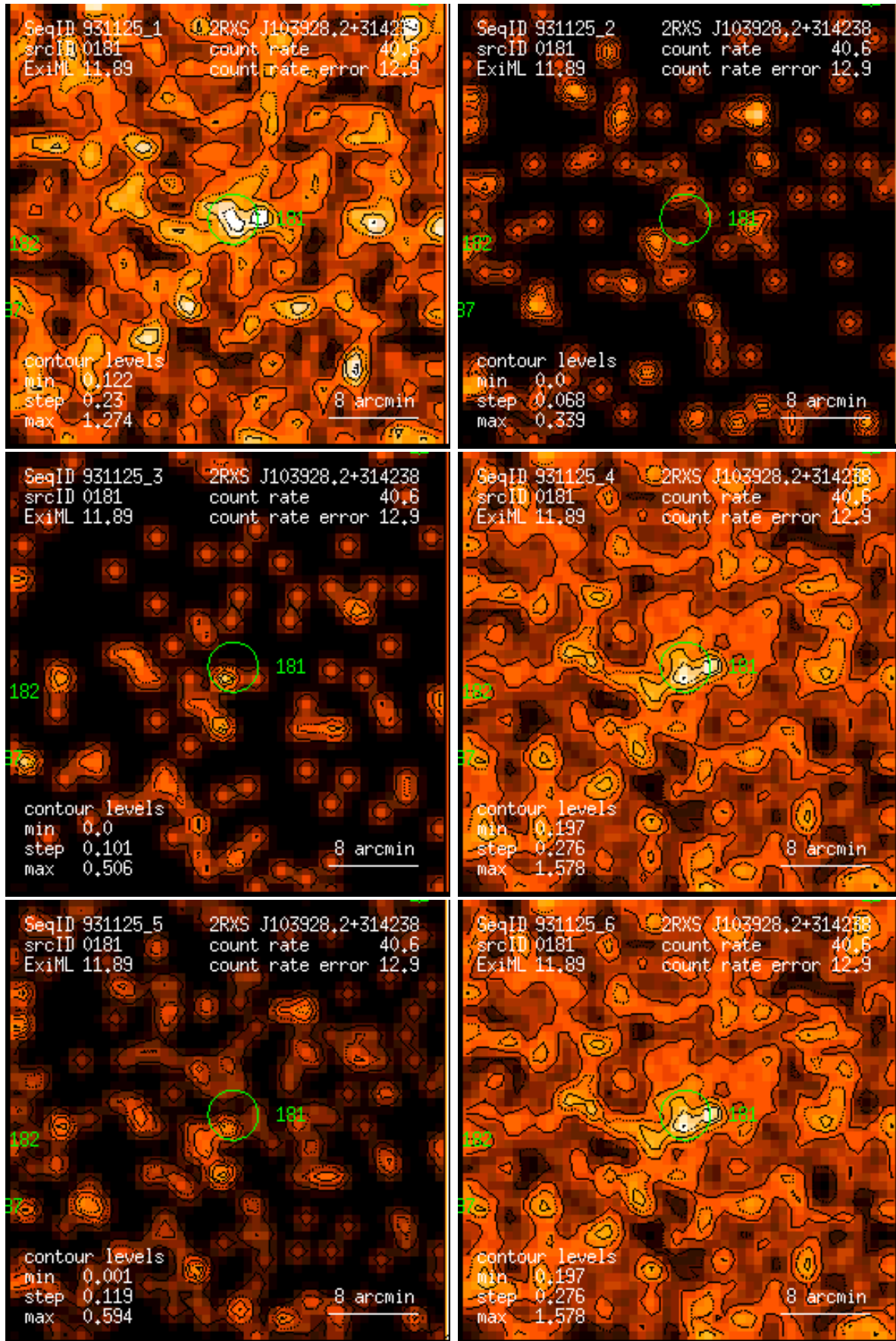
Figure 181: RASS 931125: detection 0181: band rate images, Gaussian filter: (1) PSPC channels 11 – 41, (2) 52 – 90, (3) 91 – 201, (4) 11 – 235, (5) 52 – 201, (6) 11 – 201. Broad band rates in counts/ks. Band rate contour levels in counts/ks/arcmin 2 .
