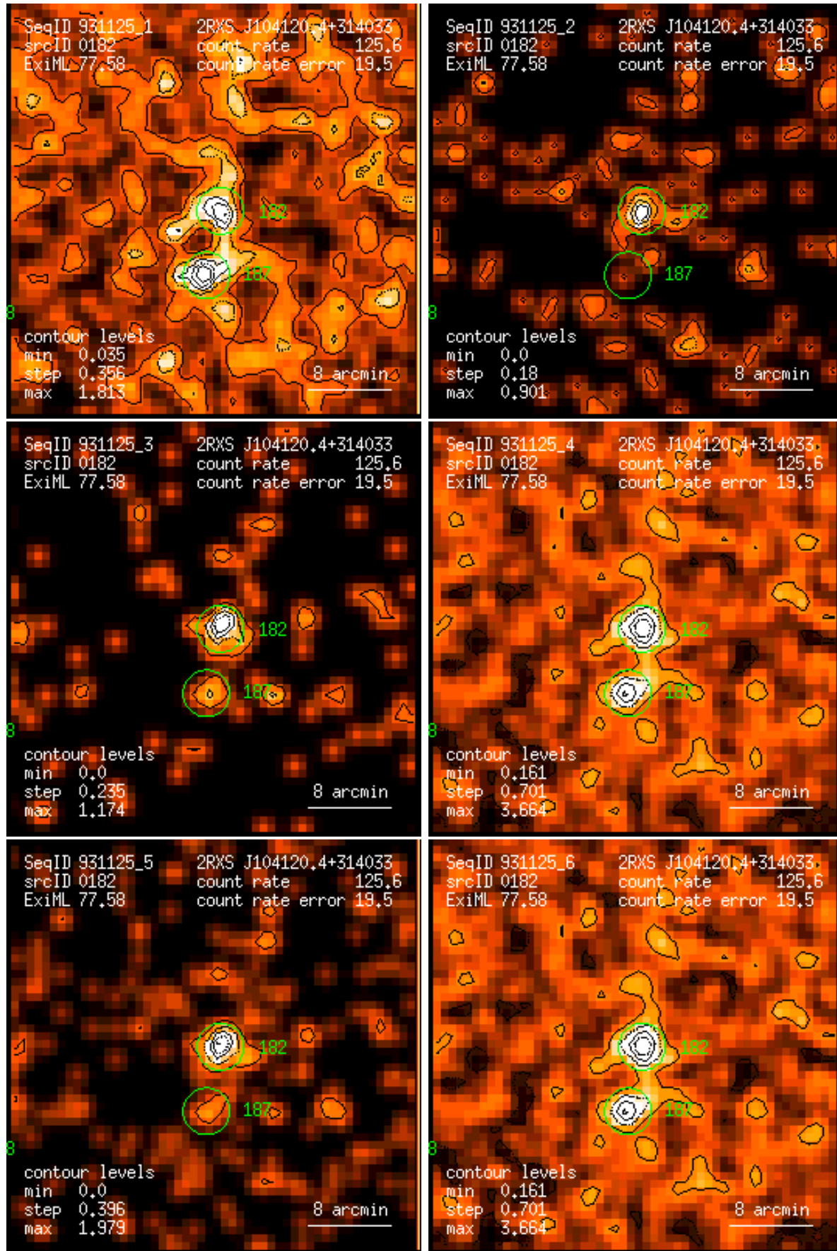
Figure 182: RASS 931125: detection 0182: band rate images, Gaussian filter: (1) PSPC channels 11 – 41, (2) 52 – 90, (3) 91 – 201, (4) 11 – 235, (5) 52 – 201, (6) 11 – 201. Broad band rates in counts/ks. Band rate contour levels in counts/ks/arcmin 2 .
