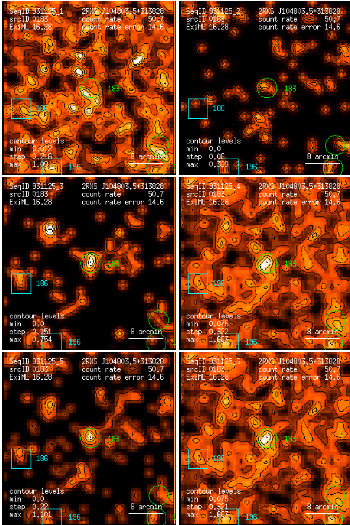
Figure 183: RASS 931125: detection 0183: band rate images, Gaussian filter: (1) PSPC channels 11 – 41, (2) 52 – 90, (3) 91 – 201, (4) 11 – 235, (5) 52 – 201, (6) 11 – 201. Broad band rates in counts/ks. Band rate contour levels in counts/ks/arcmin 2 .
