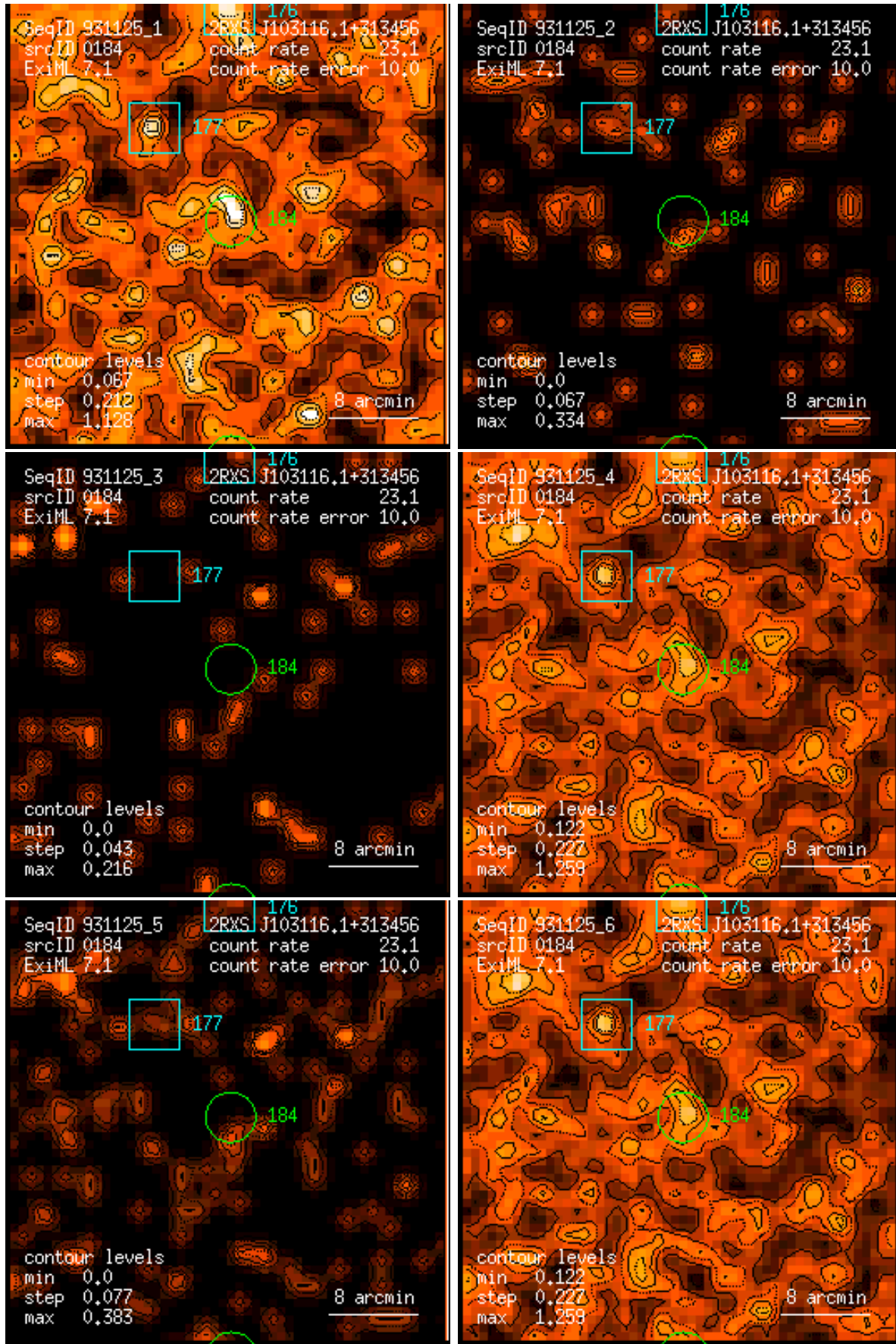
Figure 184: RASS 931125: detection 0184: band rate images, Gaussian filter: (1) PSPC channels 11 – 41, (2) 52 – 90, (3) 91 – 201, (4) 11 – 235, (5) 52 – 201, (6) 11 – 201. Broad band rates in counts/ks. Band rate contour levels in counts/ks/arcmin 2 .
