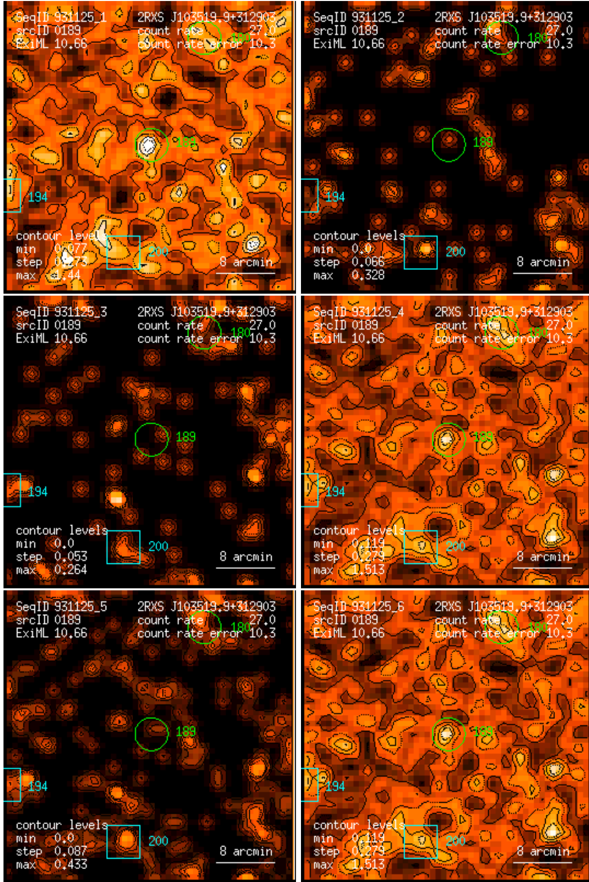
Figure 189: RASS 931125: detection 0189: band rate images, Gaussian filter: (1) PSPC channels 11 – 41, (2) 52 – 90, (3) 91 – 201, (4) 11 – 235, (5) 52 – 201, (6) 11 – 201. Broad band rates in counts/ks. Band rate contour levels in counts/ks/arcmin 2 .
