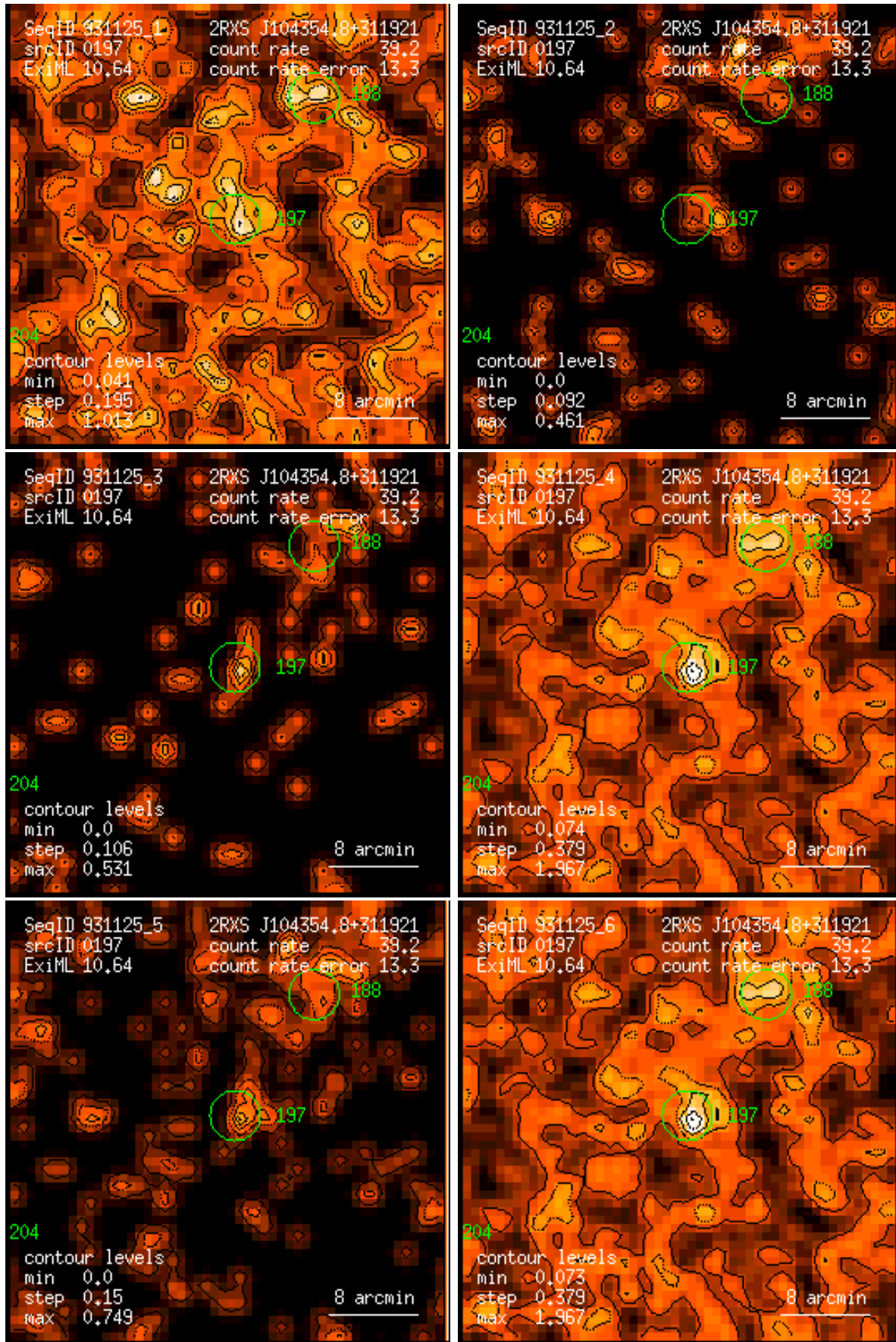
Figure 197: RASS 931125: detection 0197: band rate images, Gaussian filter: (1) PSPC channels 11 – 41, (2) 52 – 90, (3) 91 – 201, (4) 11 – 235, (5) 52 – 201, (6) 11 – 201. Broad band rates in counts/ks. Band rate contour levels in counts/ks/arcmin 2 .
