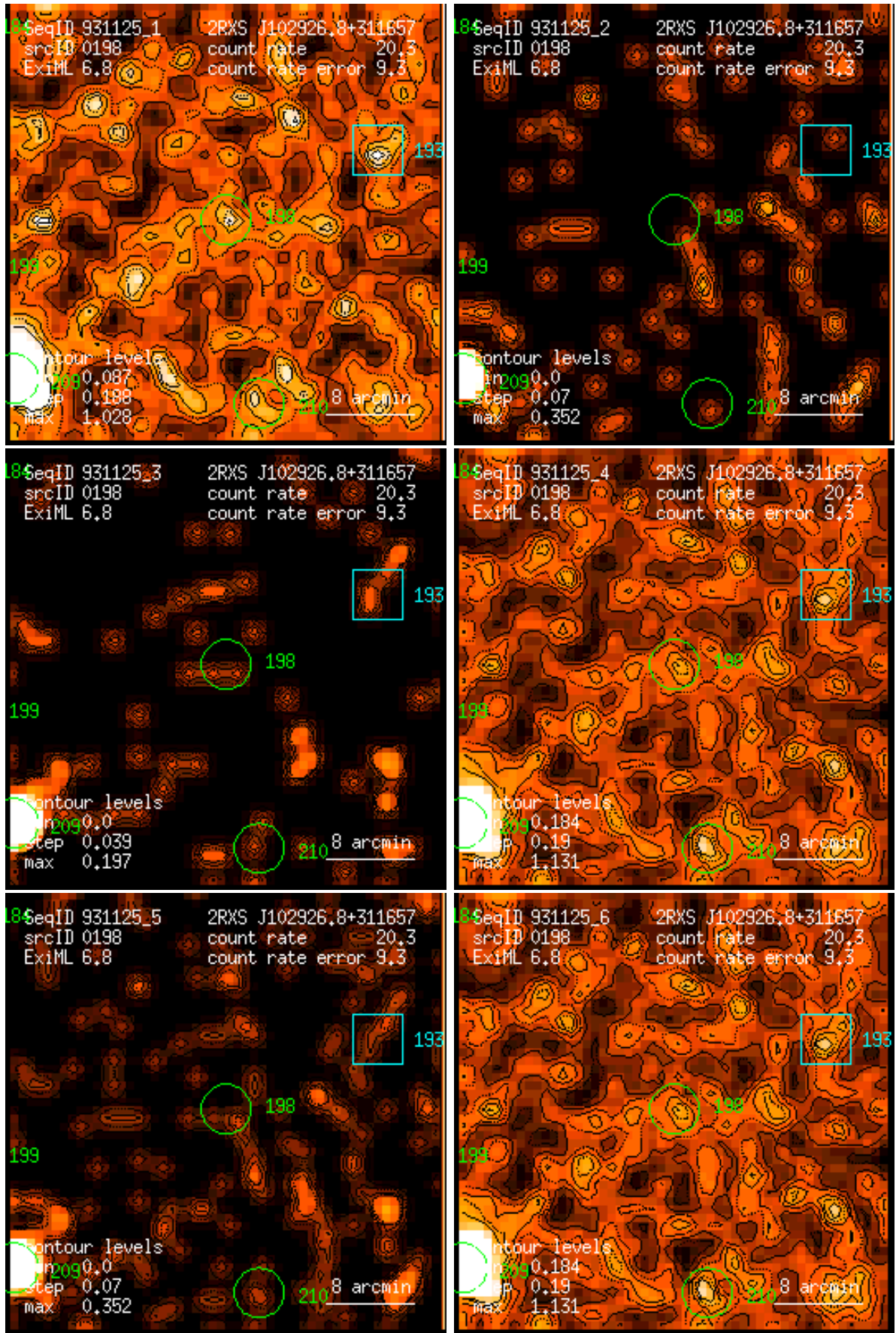
Figure 198: RASS 931125: detection 0198: band rate images, Gaussian filter: (1) PSPC channels 11 – 41, (2) 52 – 90, (3) 91 – 201, (4) 11 – 235, (5) 52 – 201, (6) 11 – 201. Broad band rates in counts/ks. Band rate contour levels in counts/ks/arcmin 2 .
