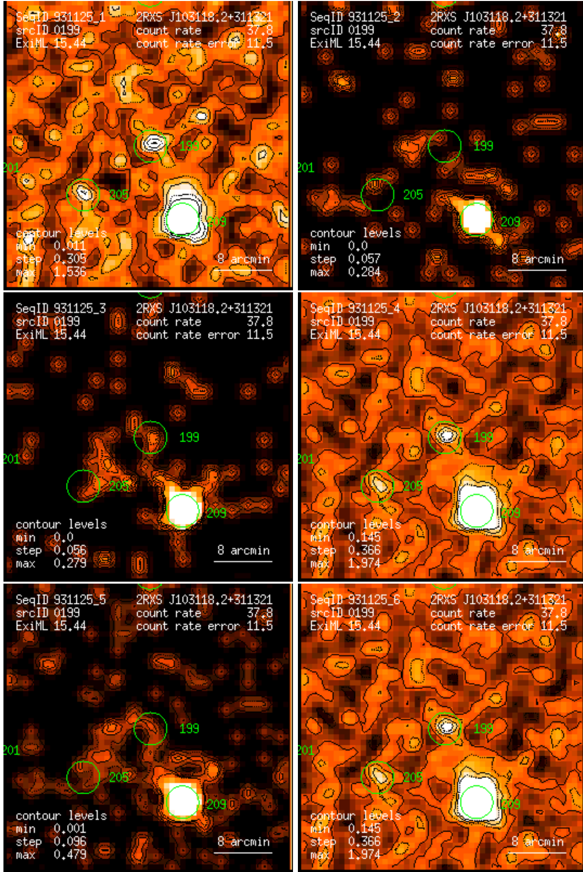
Figure 199: RASS 931125: detection 0199: band rate images, Gaussian filter: (1) PSPC channels 11 – 41, (2) 52 – 90, (3) 91 – 201, (4) 11 – 235, (5) 52 – 201, (6) 11 – 201. Broad band rates in counts/ks. Band rate contour levels in counts/ks/arcmin 2 .
