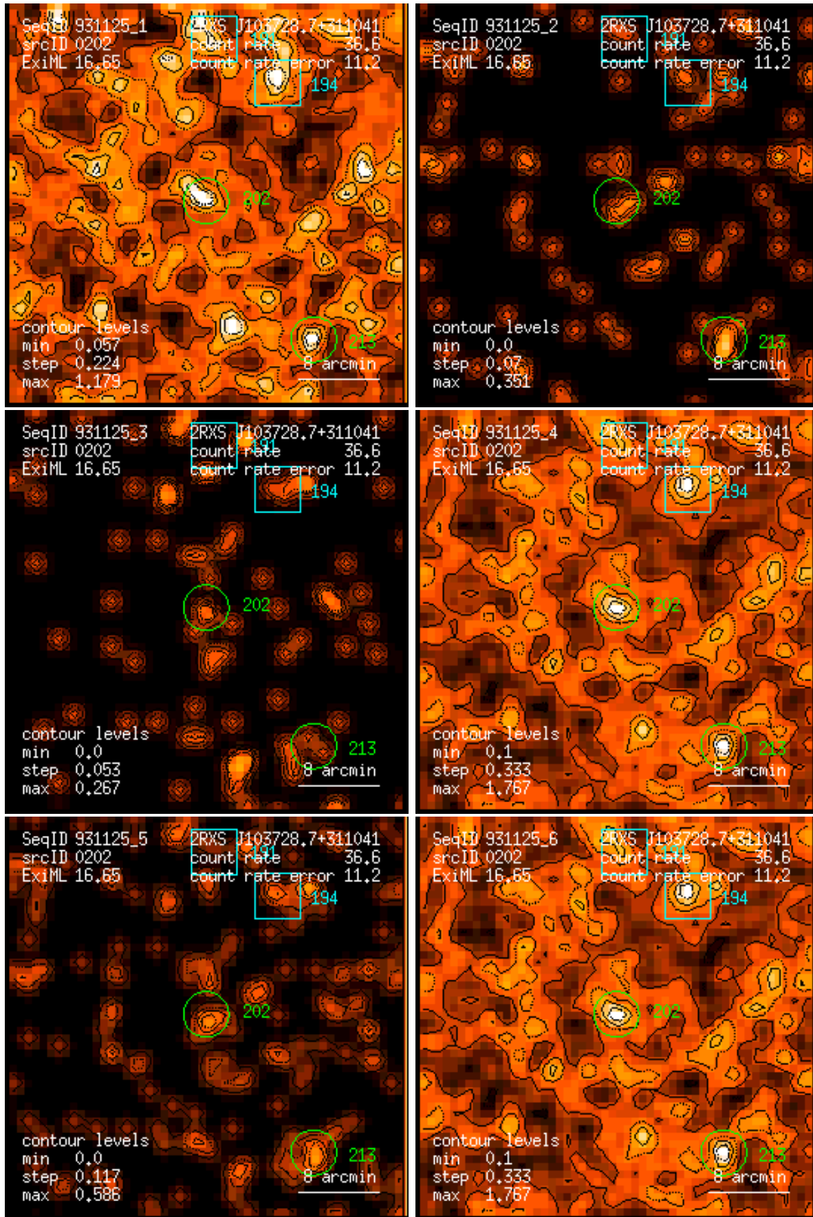
Figure 202: RASS 931125: detection 0202: band rate images, Gaussian filter: (1) PSPC channels 11 – 41, (2) 52 – 90, (3) 91 – 201, (4) 11 – 235, (5) 52 – 201, (6) 11 – 201. Broad band rates in counts/ks. Band rate contour levels in counts/ks/arcmin 2 .
