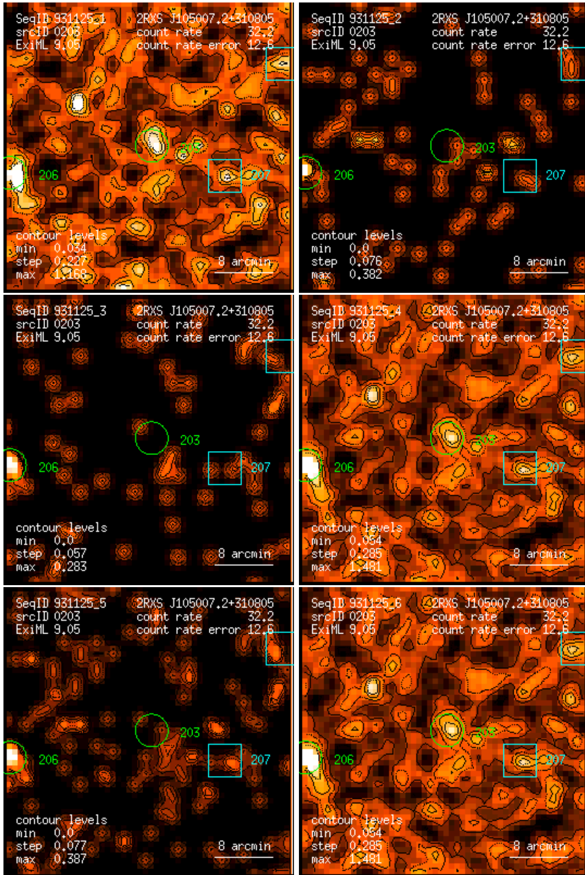
Figure 203: RASS 931125: detection 0203: band rate images, Gaussian filter: (1) PSPC channels 11 – 41, (2) 52 – 90, (3) 91 – 201, (4) 11 – 235, (5) 52 – 201, (6) 11 – 201. Broad band rates in counts/ks. Band rate contour levels in counts/ks/arcmin 2 .
