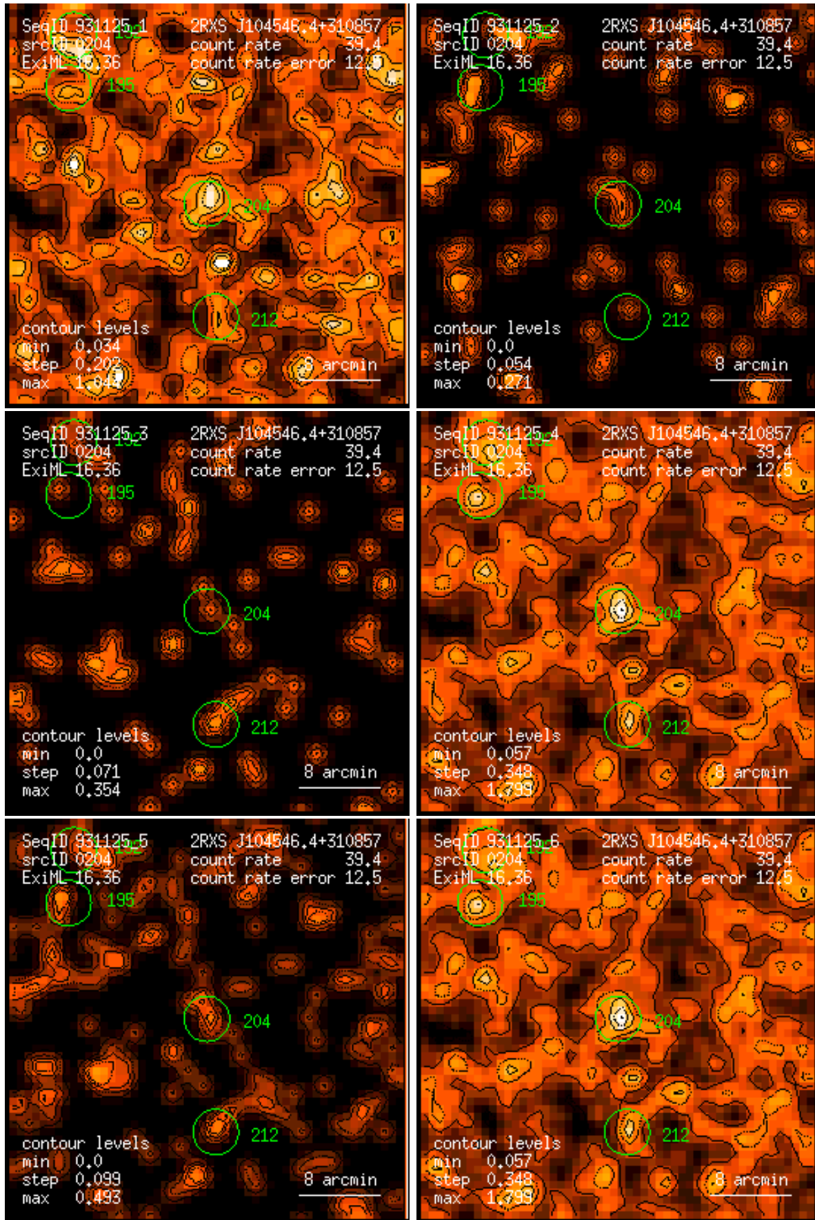
Figure 204: RASS 931125: detection 0204: band rate images, Gaussian filter: (1) PSPC channels 11 – 41, (2) 52 – 90, (3) 91 – 201, (4) 11 – 235, (5) 52 – 201, (6) 11 – 201. Broad band rates in counts/ks. Band rate contour levels in counts/ks/arcmin 2 .
