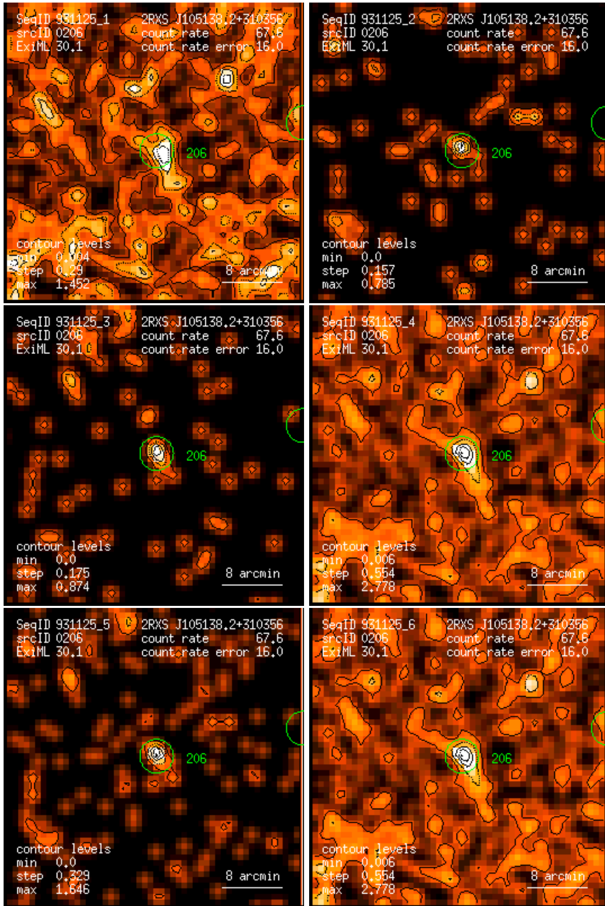
Figure 206: RASS 931125: detection 0206: band rate images, Gaussian filter: (1) PSPC channels 11 – 41, (2) 52 – 90, (3) 91 – 201, (4) 11 – 235, (5) 52 – 201, (6) 11 – 201. Broad band rates in counts/ks. Band rate contour levels in counts/ks/arcmin 2 .
