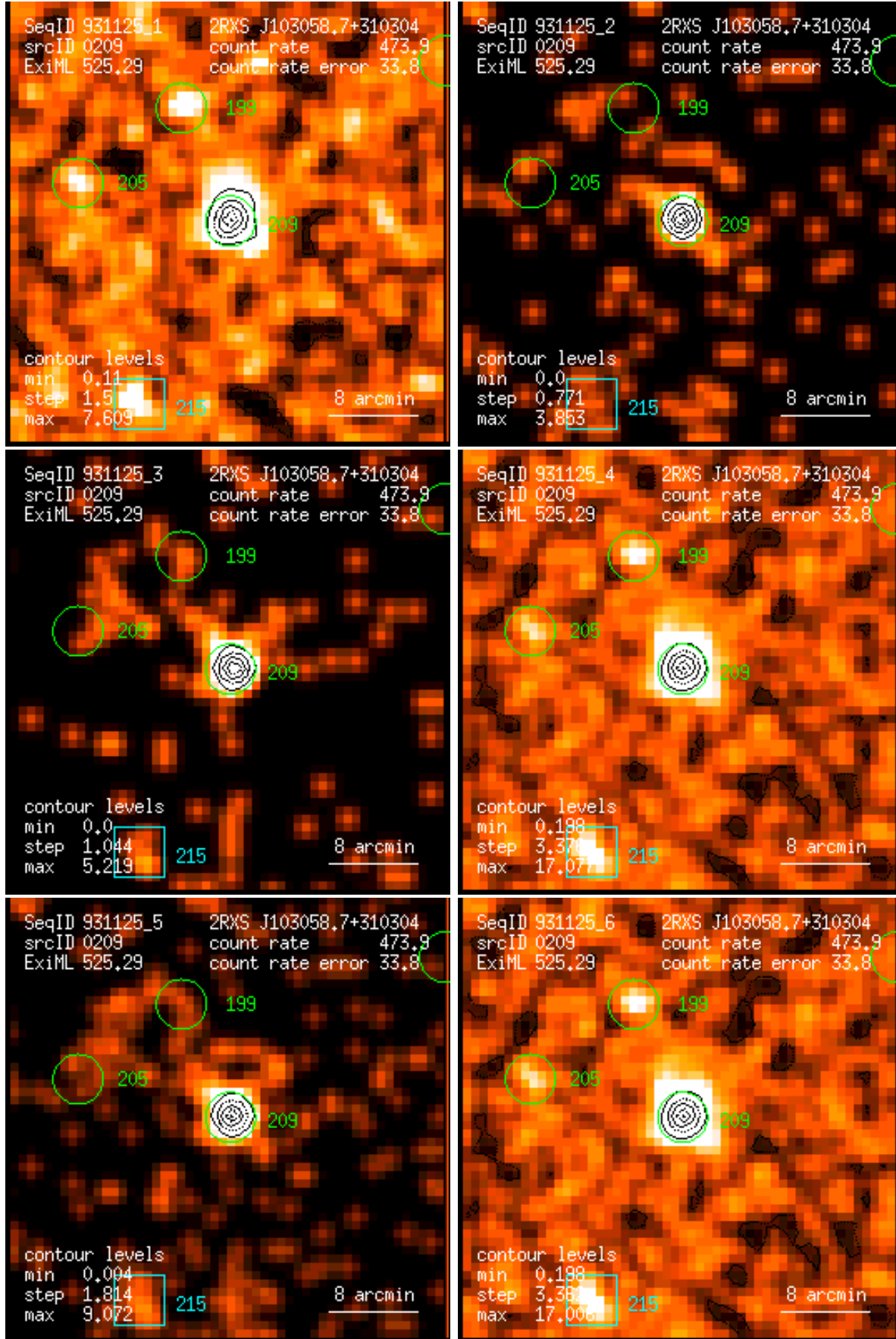
Figure 209: RASS 931125: detection 0209: band rate images, Gaussian filter: (1) PSPC channels 11 – 41, (2) 52 – 90, (3) 91 – 201, (4) 11 – 235, (5) 52 – 201, (6) 11 – 201. Broad band rates in counts/ks. Band rate contour levels in counts/ks/arcmin 2 .
